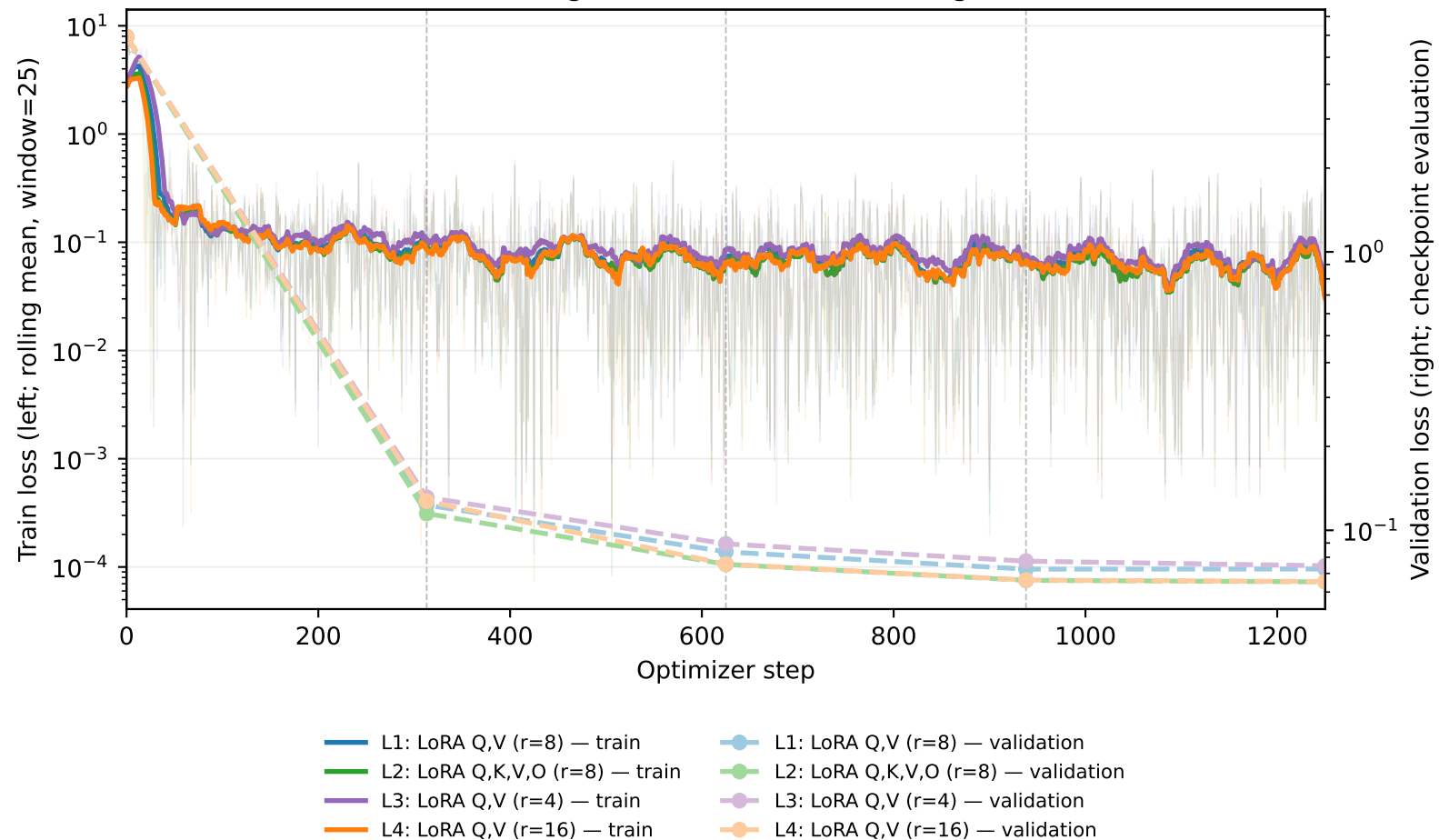
RQ2: LoRA target-module and rank configurations
