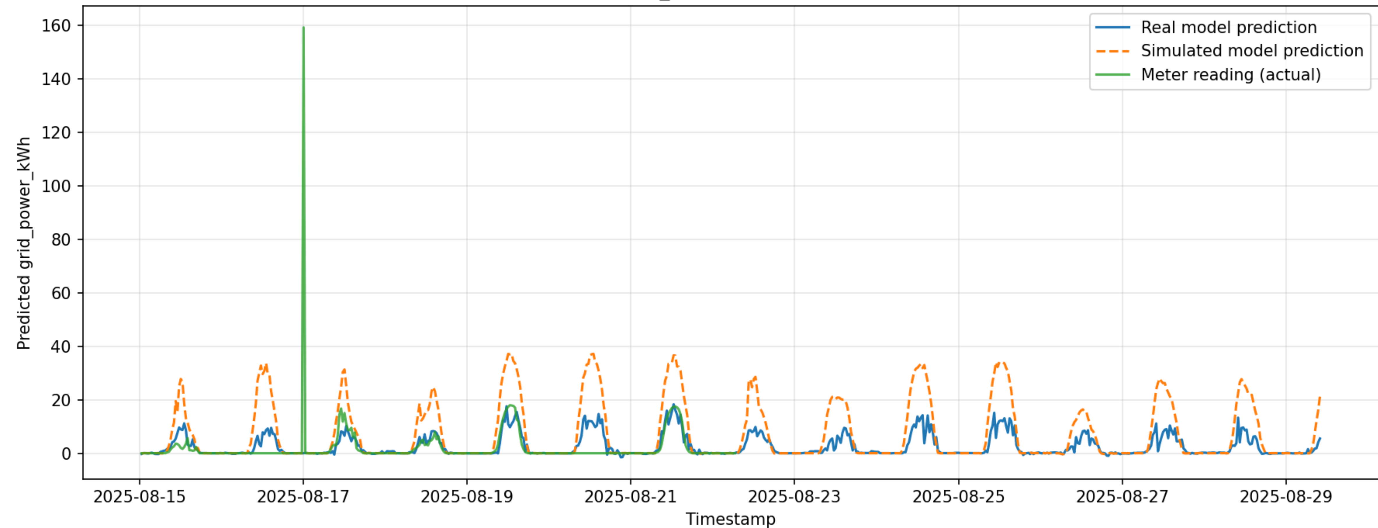
Forecast comparison — solar.bun_hsc#realenergyintothelead#kwh (BUNDOORA)
