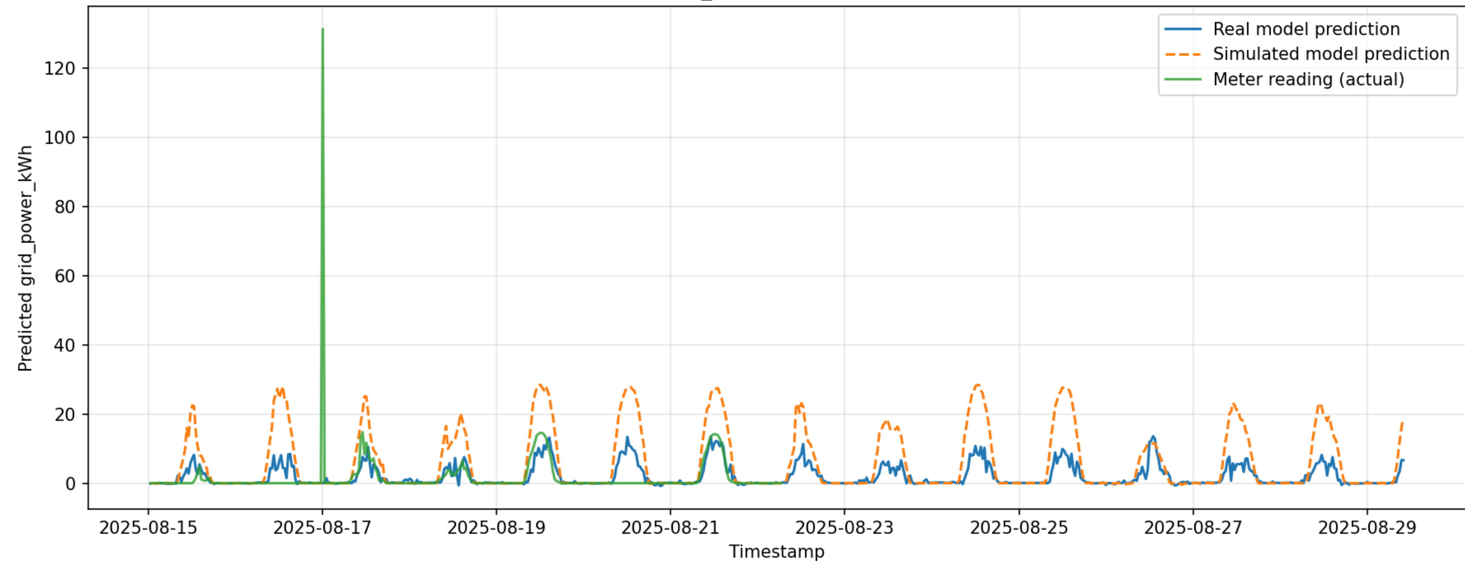
Forecast comparison — solar.bun_cs1#realenergyintothelead#kwh (BUNDOORA)
