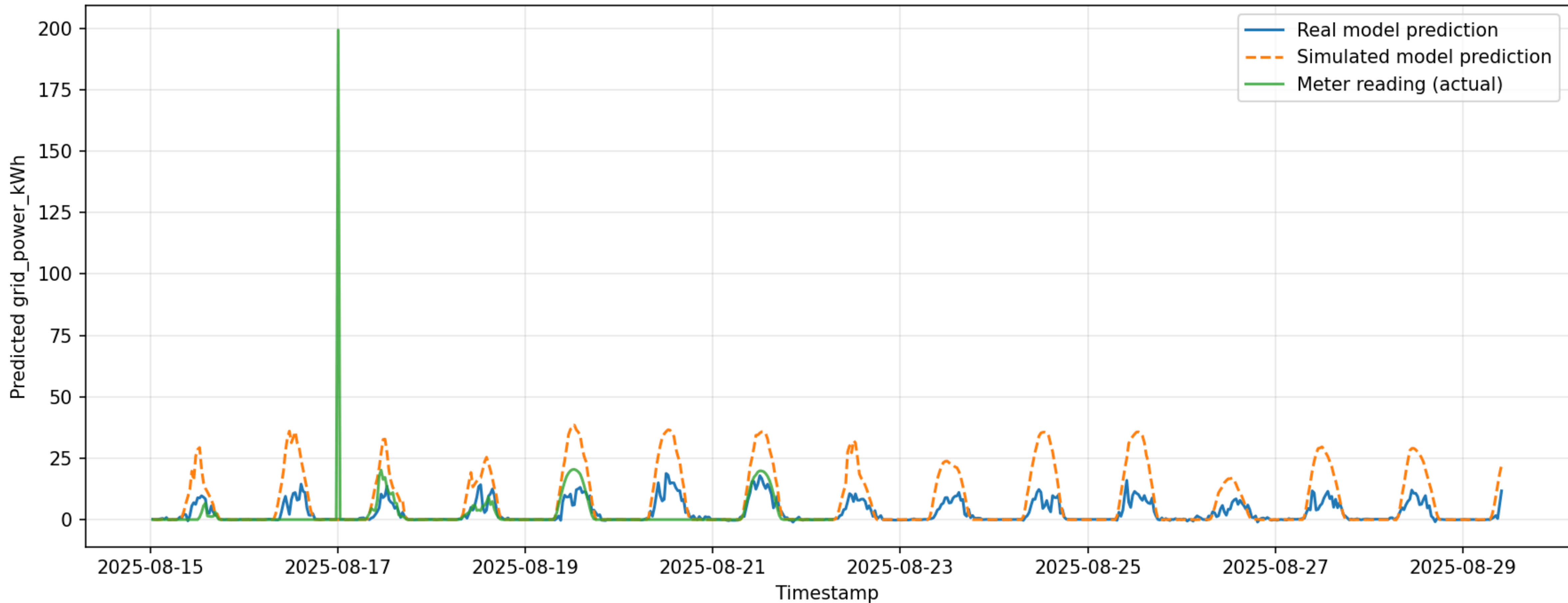
Forecast comparison — solar.bun_bg#realenergyintothe load#kwh (BUNDOORA)
