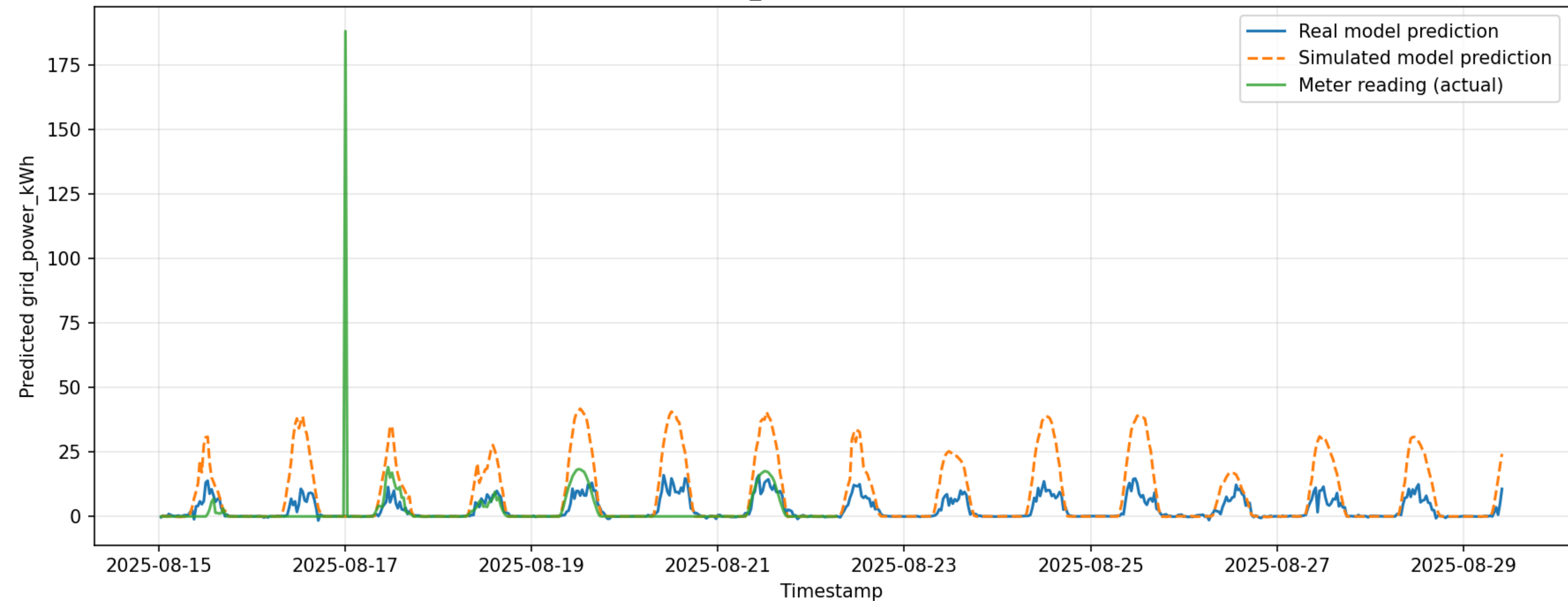
Forecast comparison — solar.bun_hs3#realenergyintotheload#kwh (BUNDOORA)
