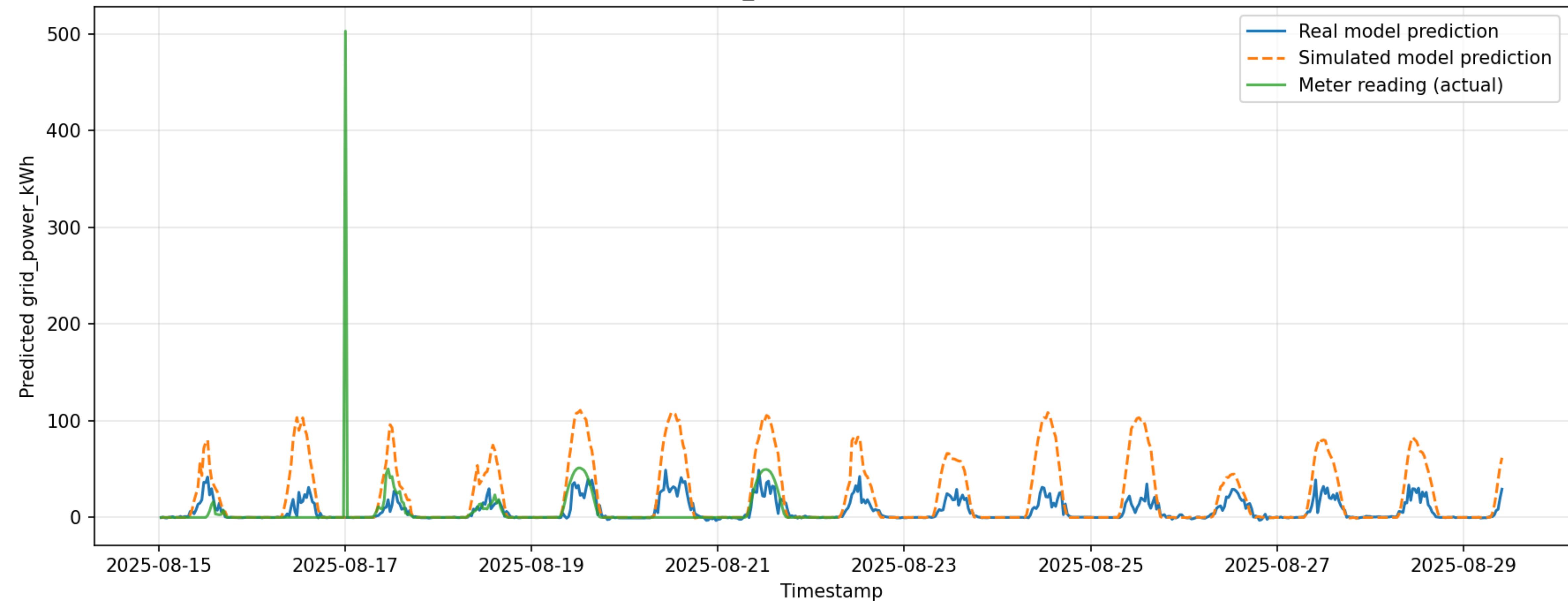
Forecast comparison — solar.bun_dmw#realenergyintotheload#kwh (BUNDOORA)
