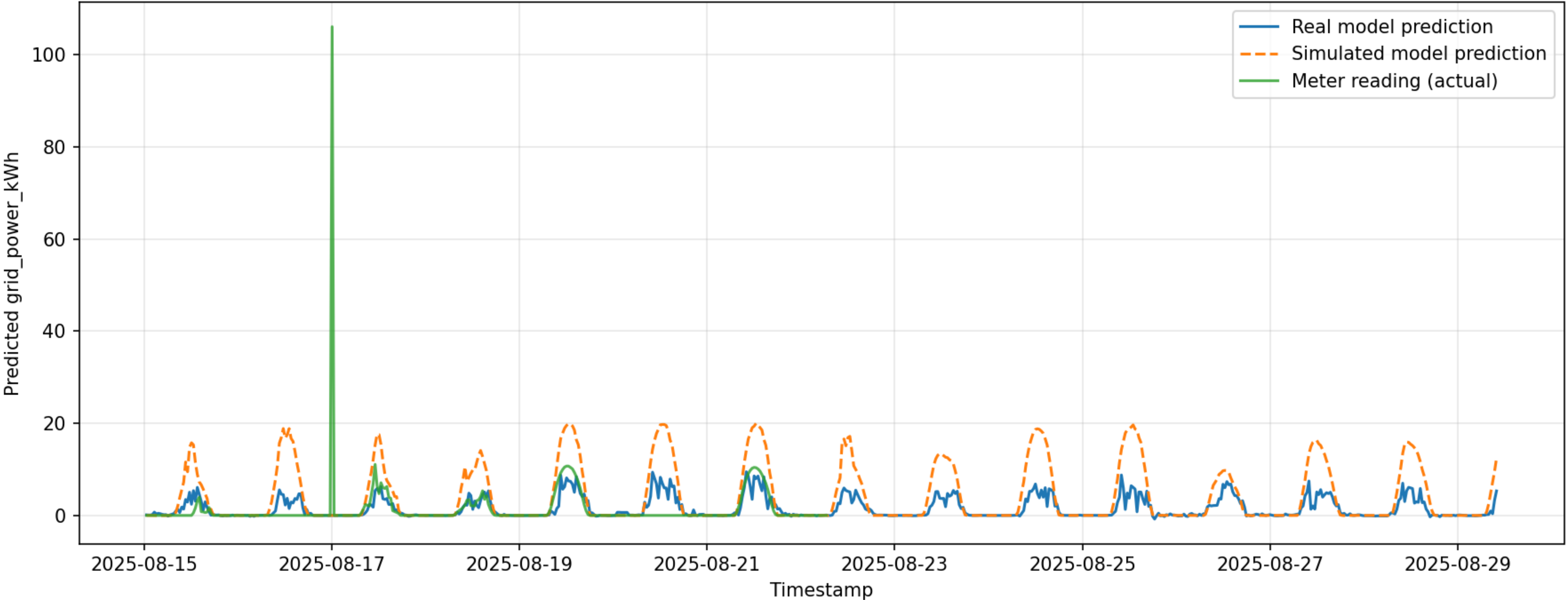
Forecast comparison — solar.bun_lims1#realenergyintotheload#kwh (BUNDOORA)
