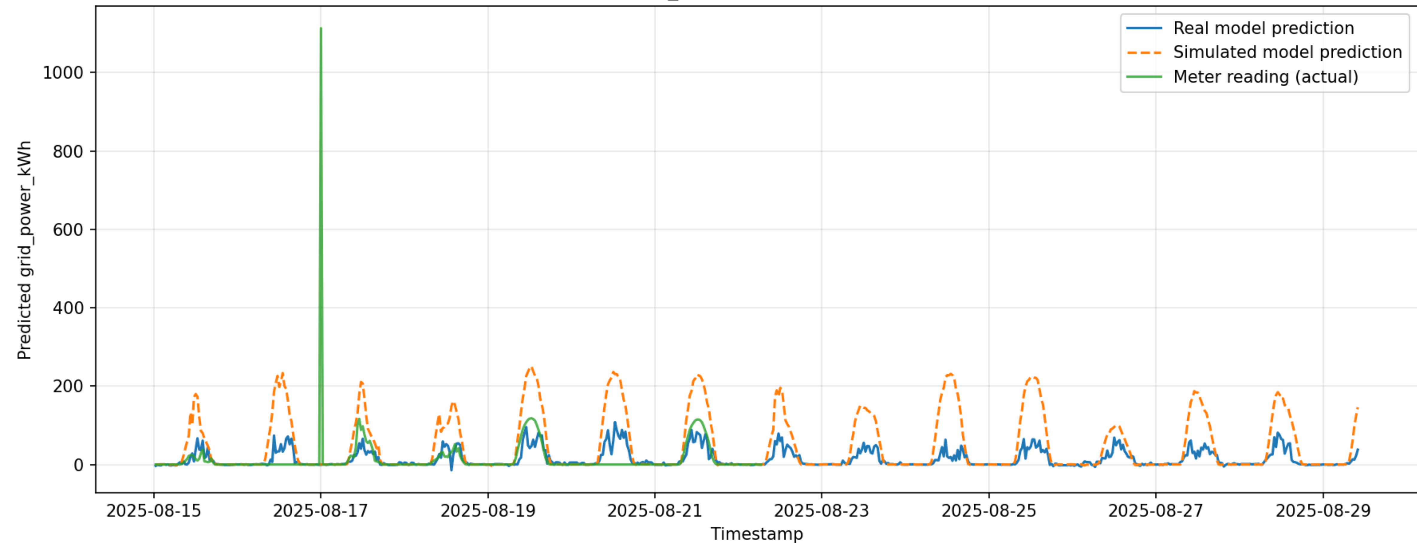
Forecast comparison — solar.bun_library#realenergyintotheload#kwh (BUNDOORA)
