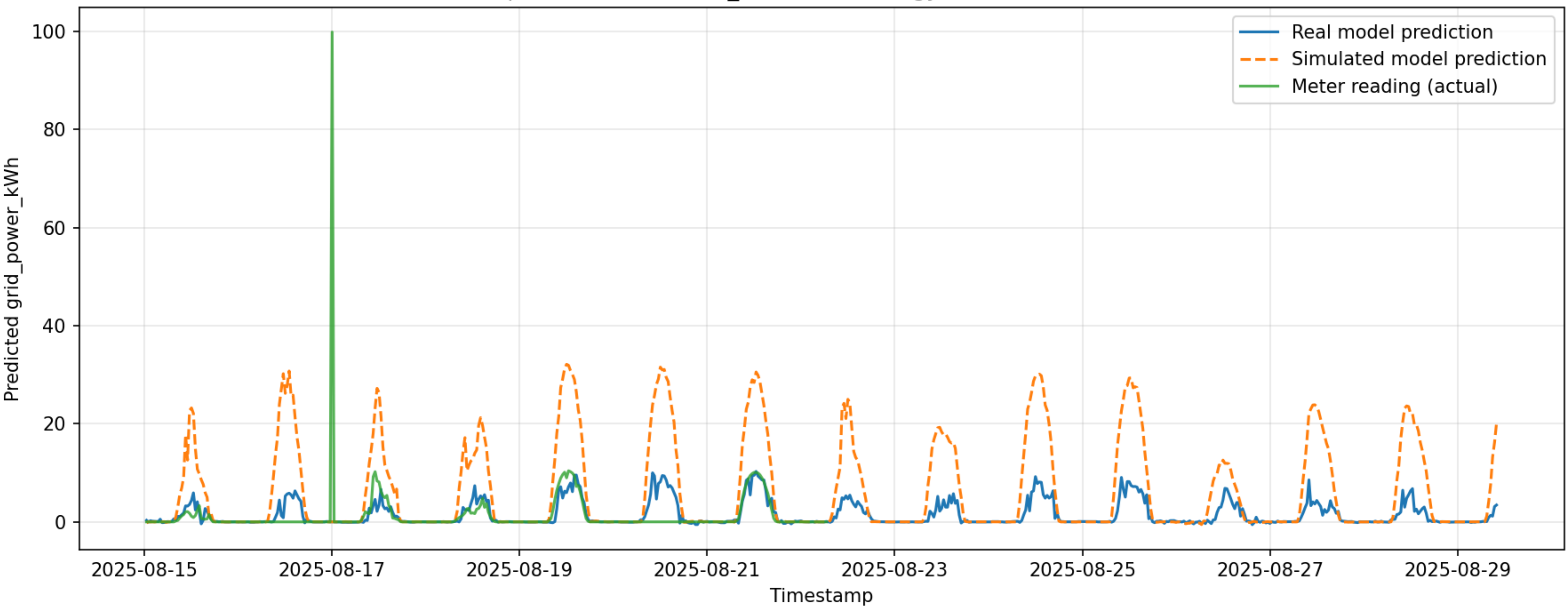
Forecast comparison — solar.bun_union#realenergyintothelead#kwh (BUNDOORA)
