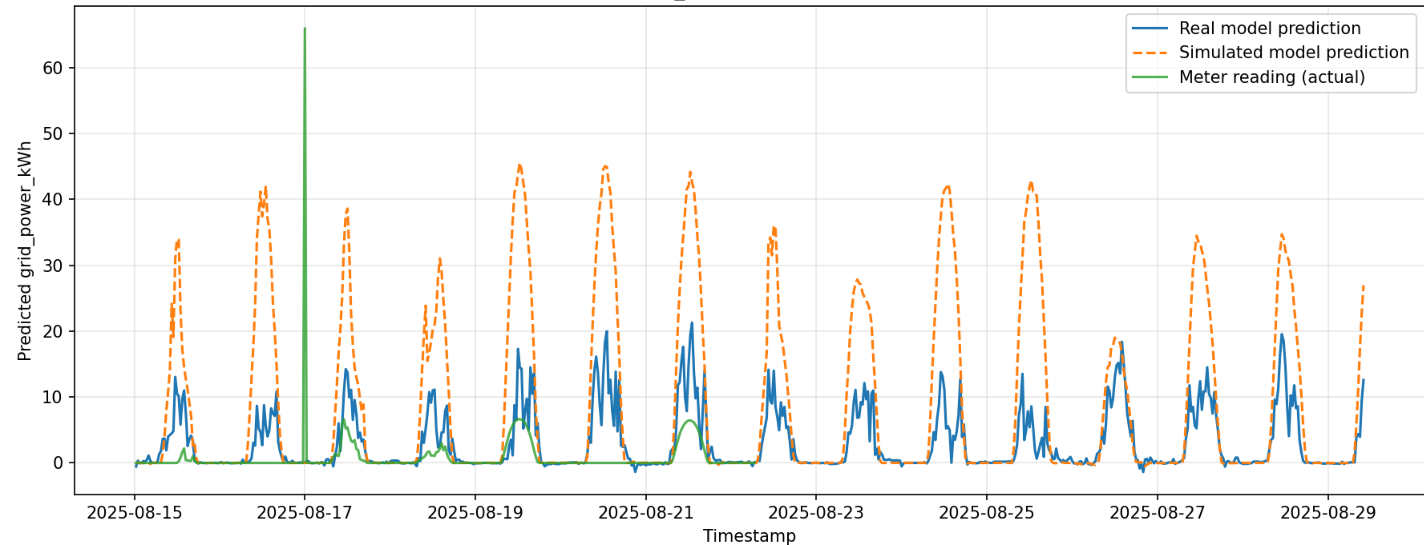
Forecast comparison — solar.bun_hu3#realenergyintothelead#kwh (BUNDOORA)
