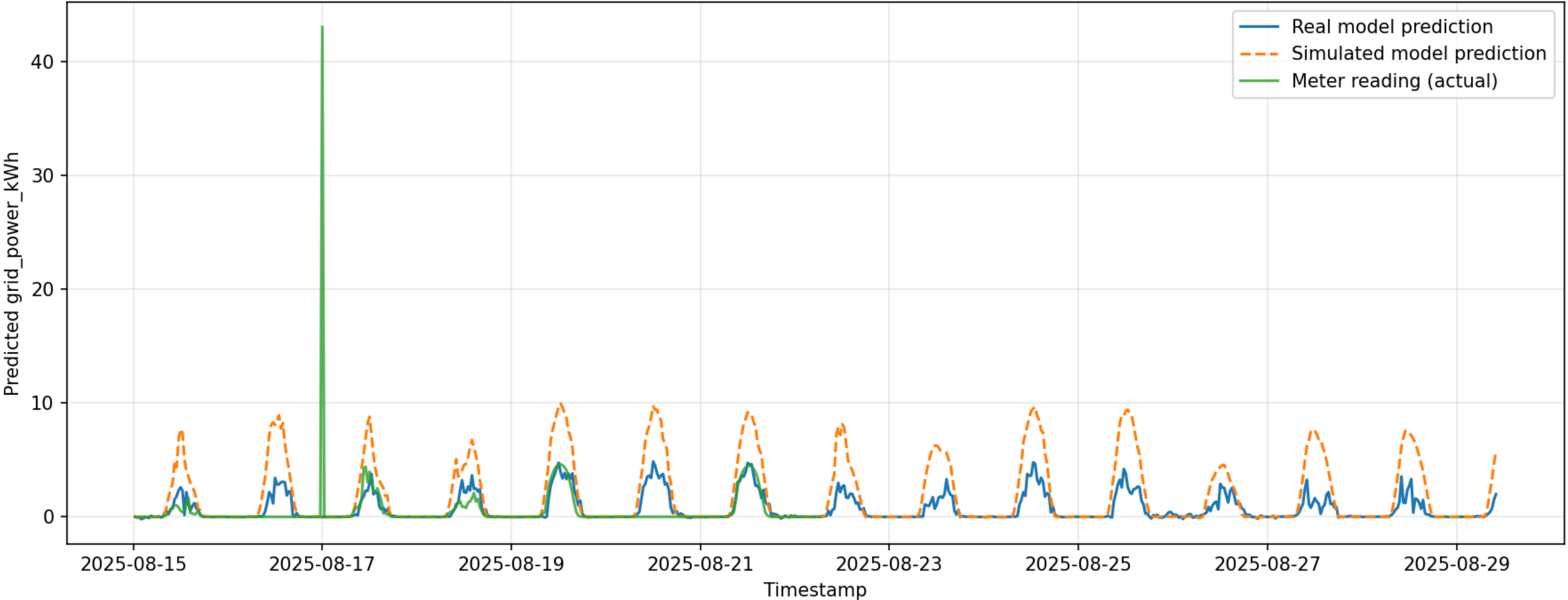
Forecast comparison — solar.bun_lwso#realenergyintothelead#kwh (BUNDOORA)
