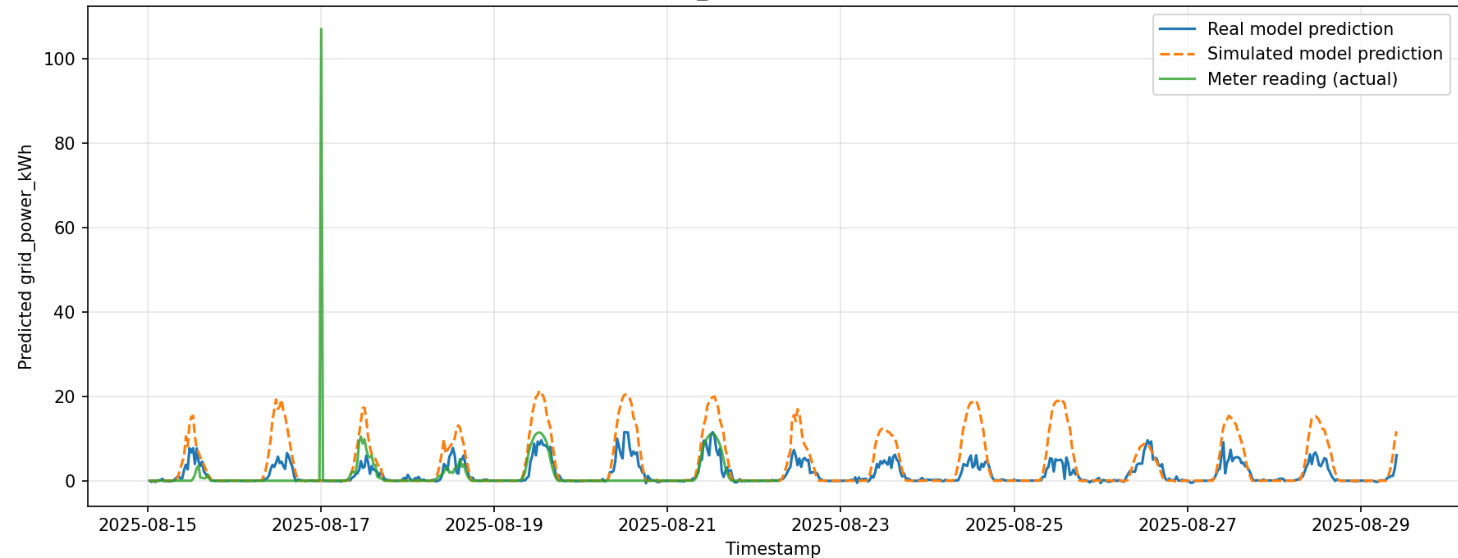
Forecast comparison — solar.bun_hs2#realenergyintothelead#kwh (BUNDOORA)
