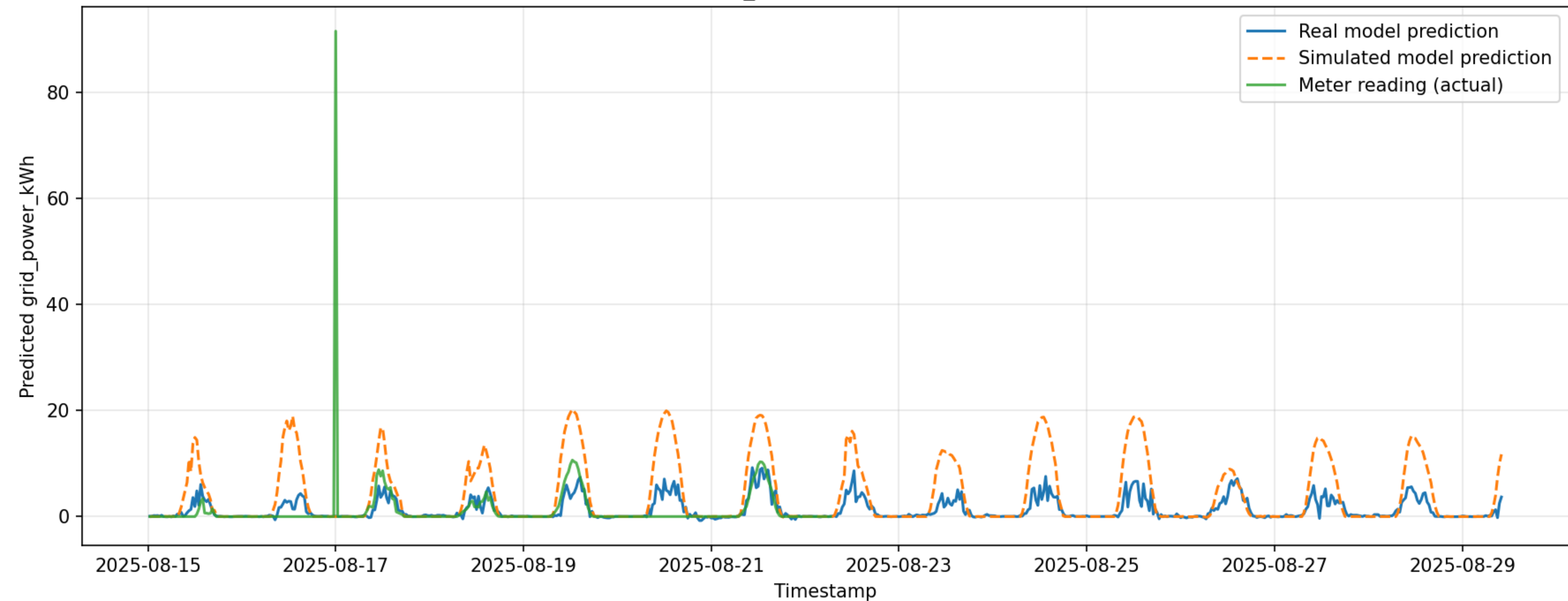
Forecast comparison — solar.bun_ps2#realenergyintotheload#kwh (BUNDOORA)
