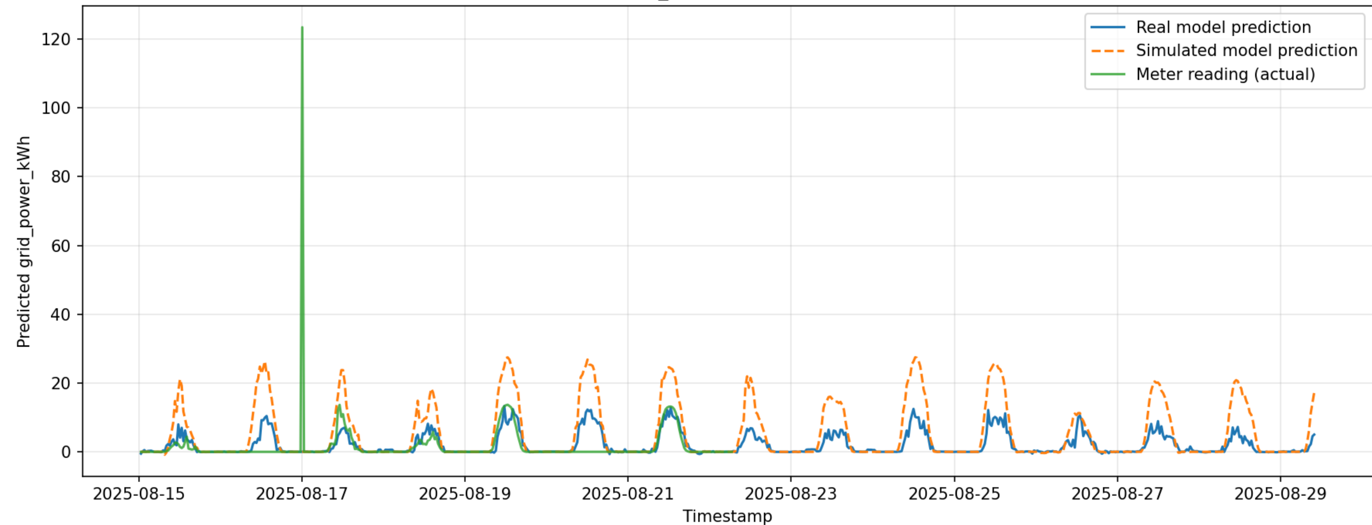
Forecast comparison — solar.bun_mc#realenergyintothe load#kwh (BUNDOORA)
