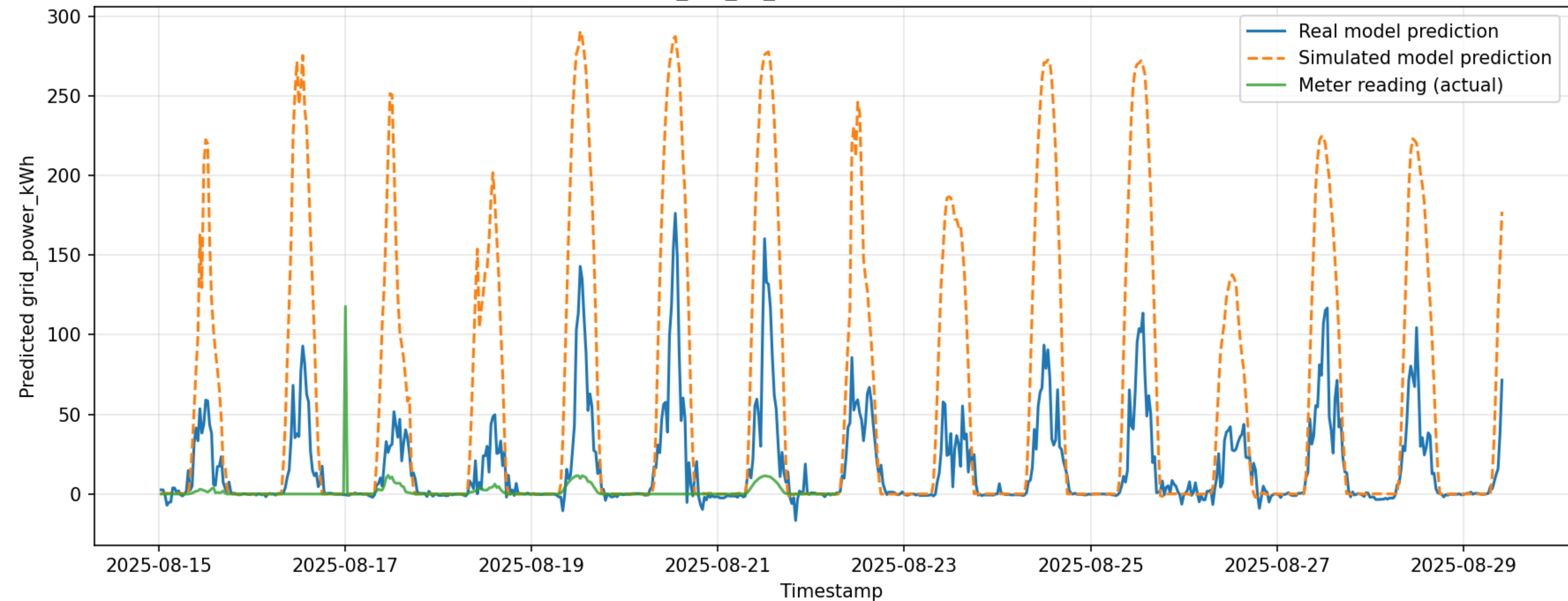
Forecast comparison — solar.bun_ltss_pv_lgcmeter#realenergyintothelead#kwh (BUNDOORA)
