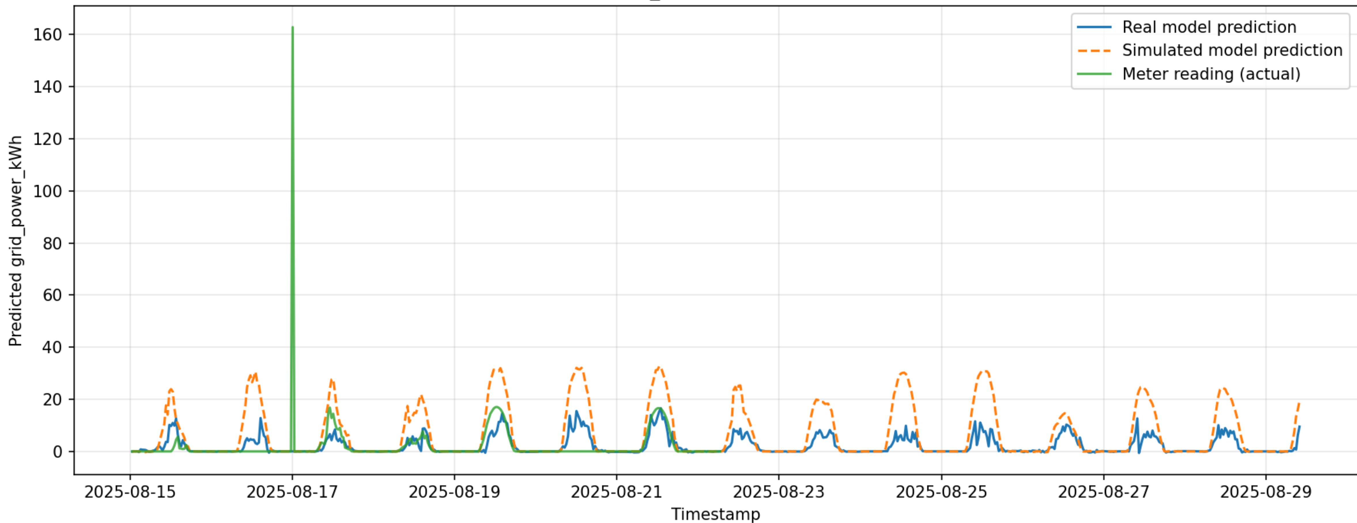
Forecast comparison — solar.bun_tlc#realenergyintothelead#kwh (BUNDOORA)
