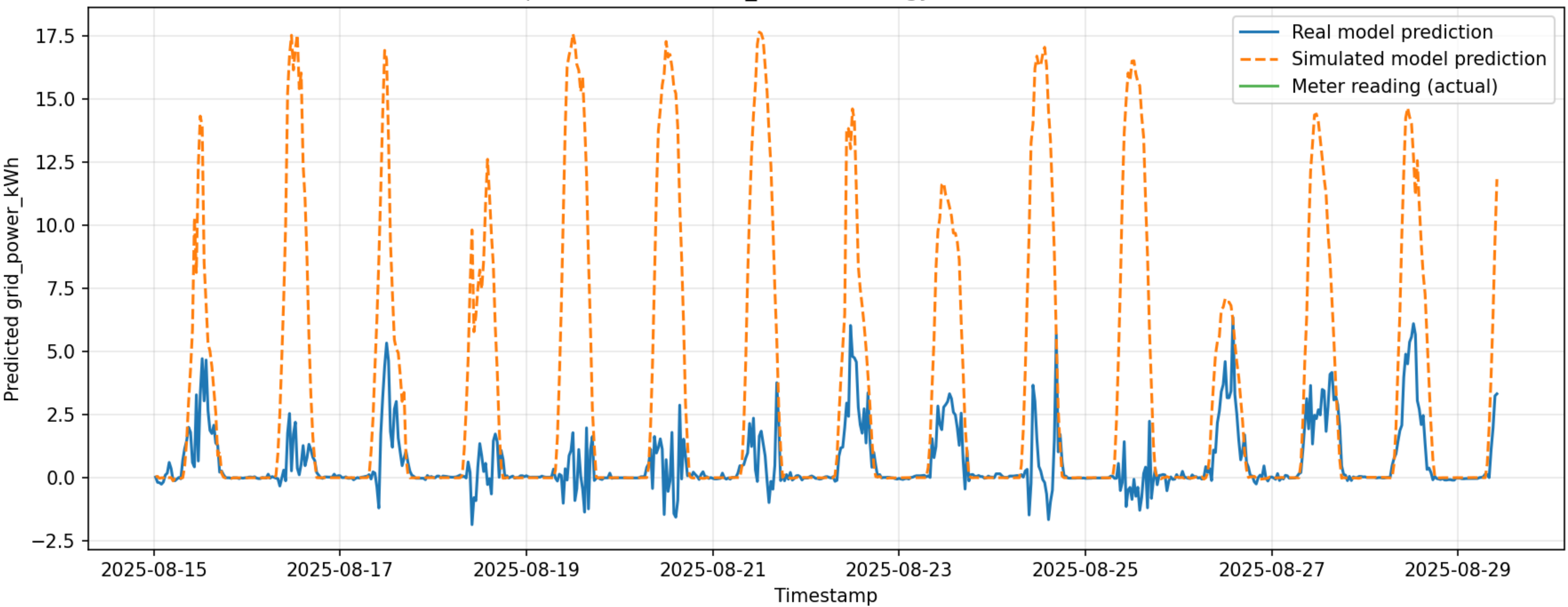
Forecast comparison — solar.bun_rd2#realenergyintothe load#kwh (BUNDOORA)
