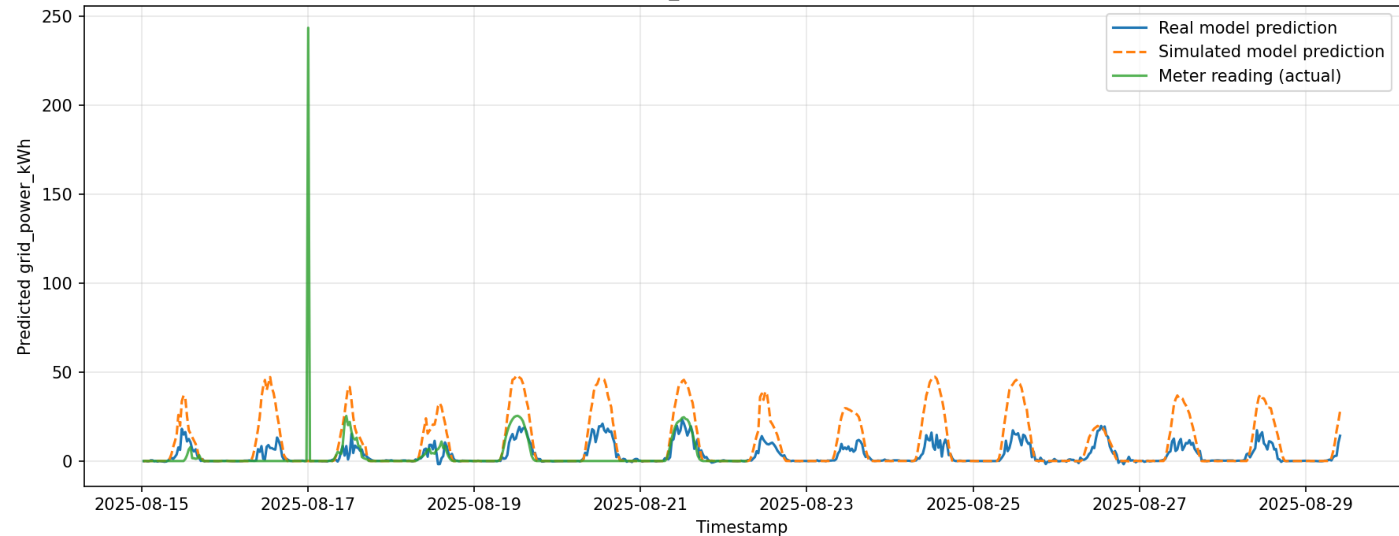
Forecast comparison — solar.bun_hs1#realenergyintothelead#kwh (BUNDOORA)
