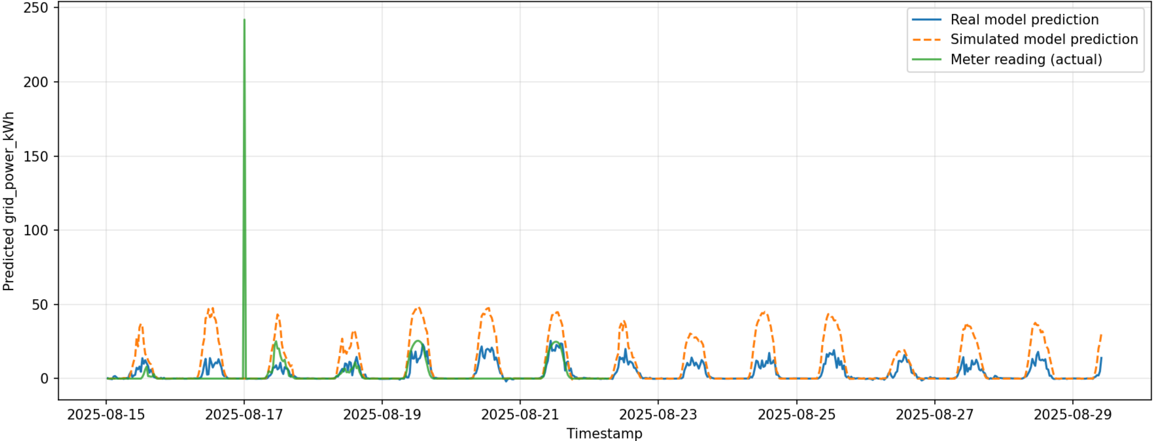
Forecast comparison — solar.bun_pe#realenergyintotheload#kwh (BUNDOORA)
