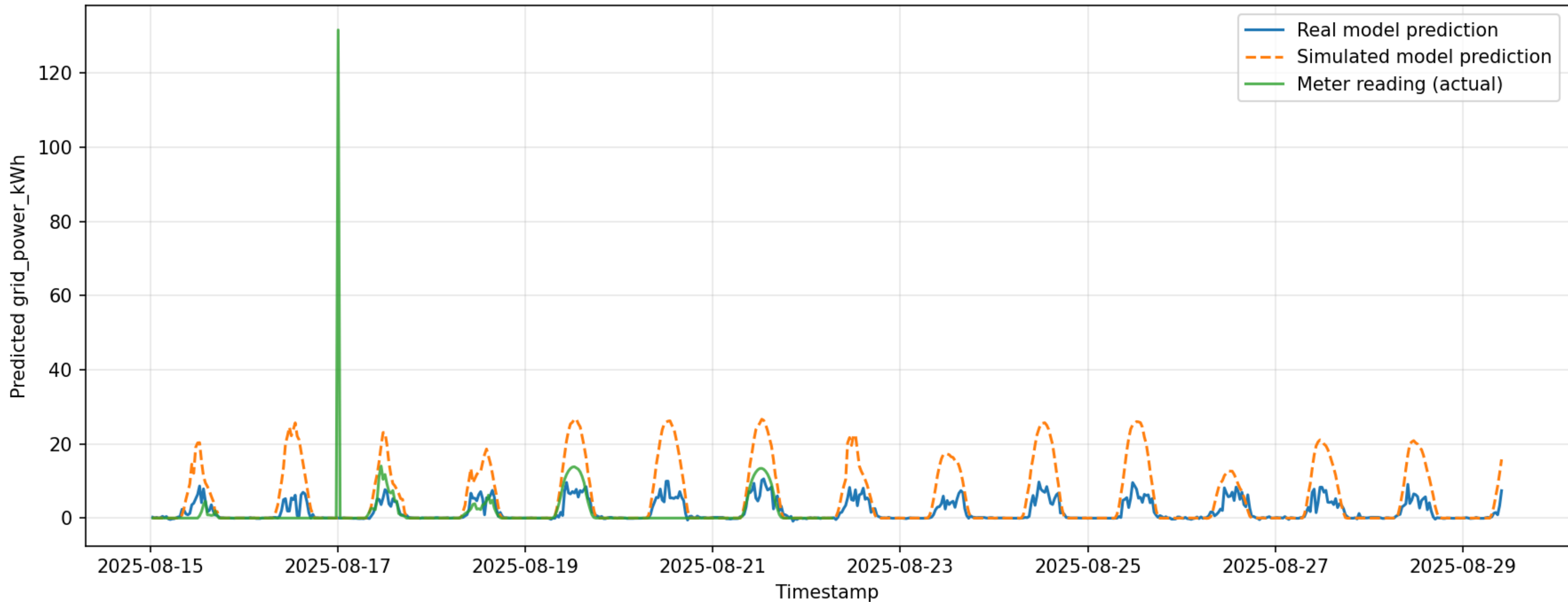
Forecast comparison — solar.bun_rlr#realenergyintothe load#kwh (BUNDOORA)
