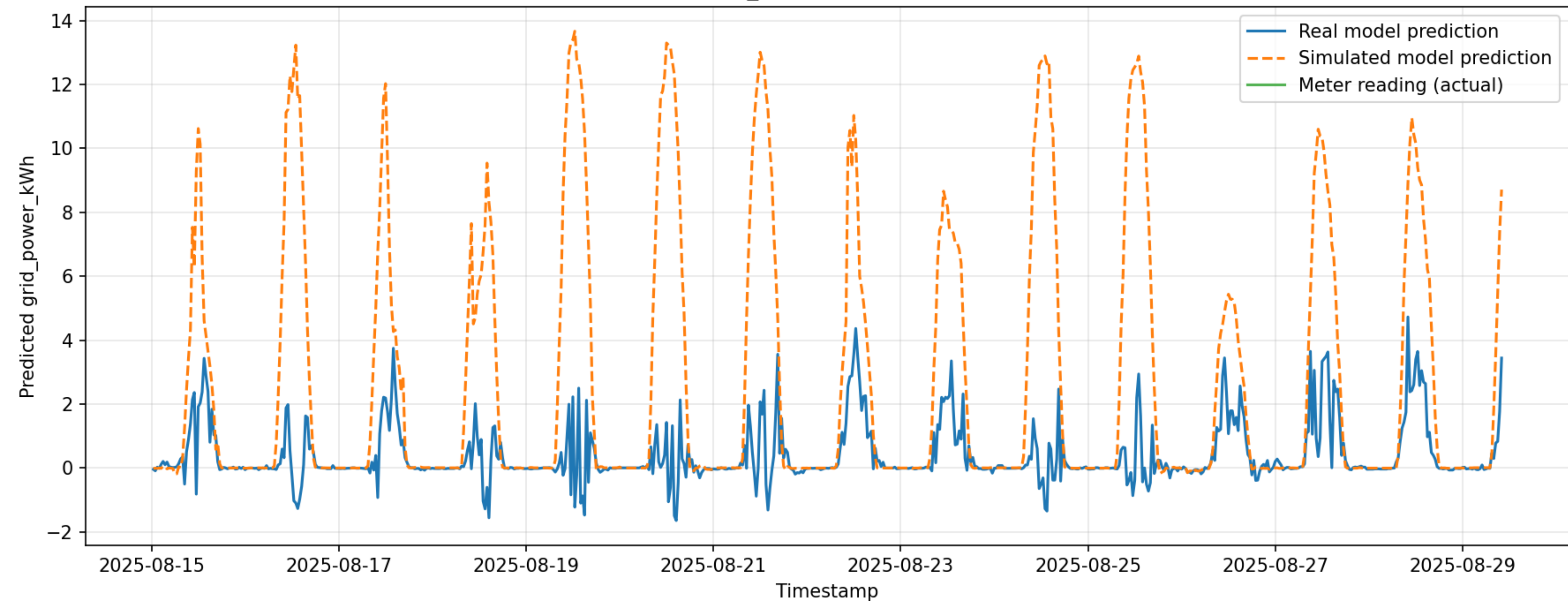
Forecast comparison — solar.bun_rd1#realenergyintothe load#kwh (BUNDOORA)
