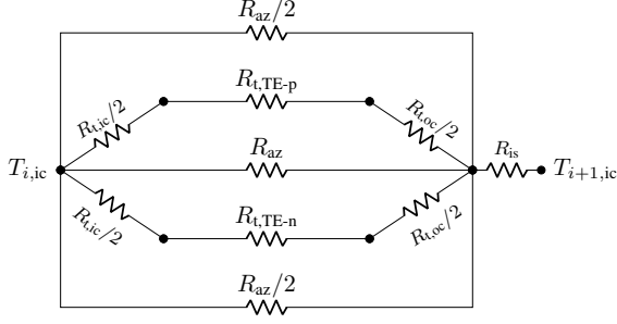
Figure 10: Resistor network between two adjacent interconnector nodes.
