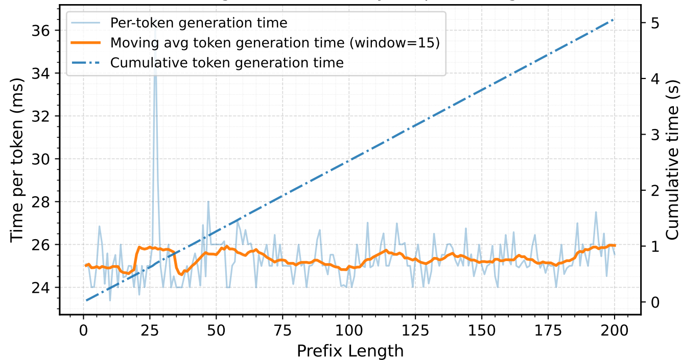
Token generation latency vs. prefix length
