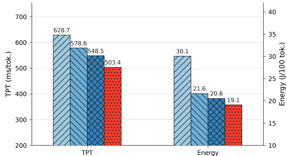
HumanEval
