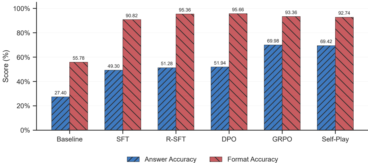
MATH Overall Metrics Across Training Stages
