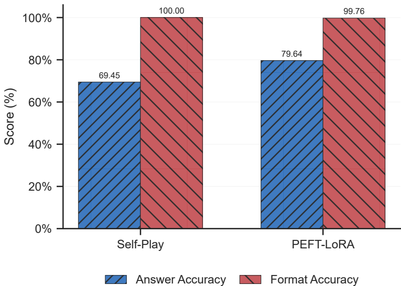
ScienceQA Nature Science Subset Overall Metrics
