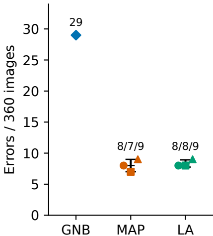
A Recognition
