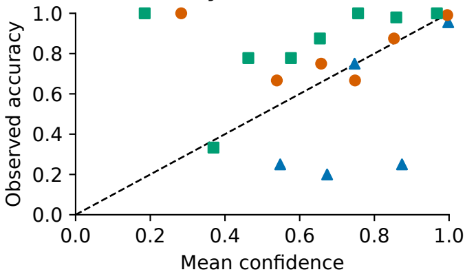
A Reliability (seed 11)
