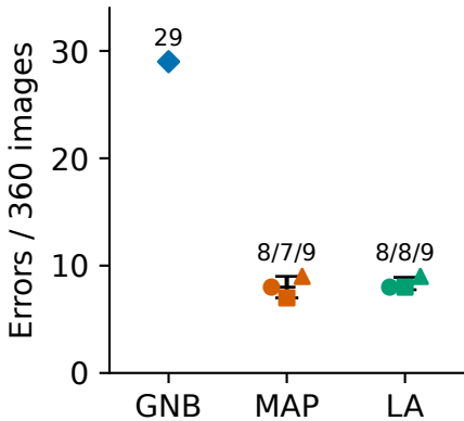
A Recognition
