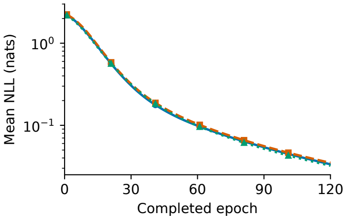
A Training
