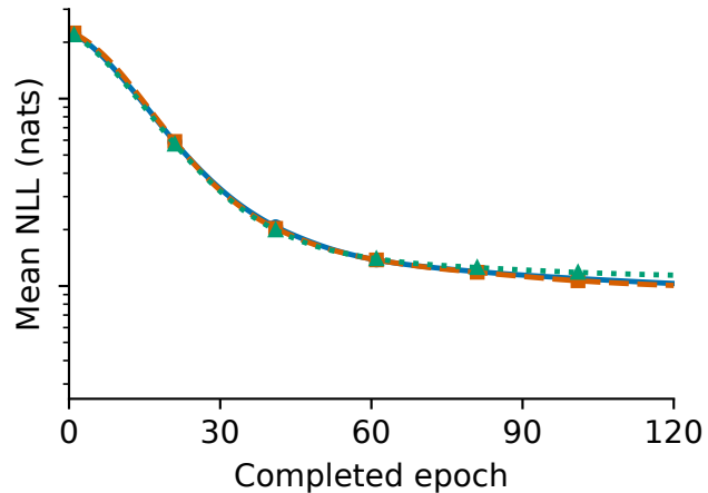
B Validation
