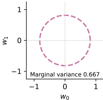
B Diagonal precision
