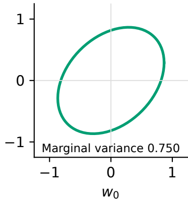
A Full covariance
