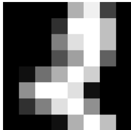
idx 1078: 0 -> 2 confidence 0.44
