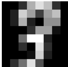
idx 1118: 3 -> 8 confidence 0.39
