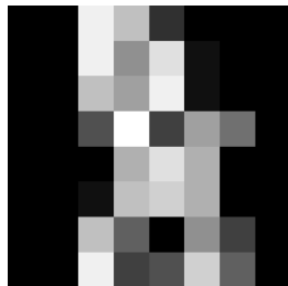
idx 1149: 8 -> 1 confidence 0.68
