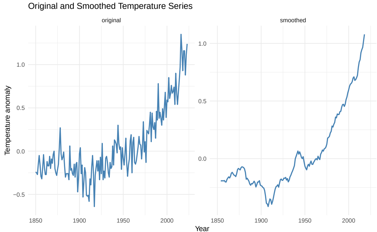
Figure 4.29.: A simple comparison between the original and smoothed versions of the same series.
