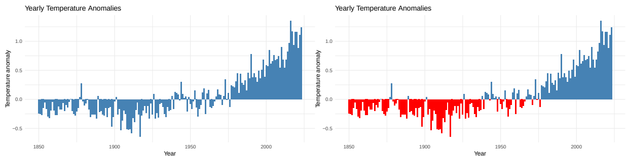
Figure 4.30.: A bar chart emphasizing positive and negative yearly temperature anomalies.
