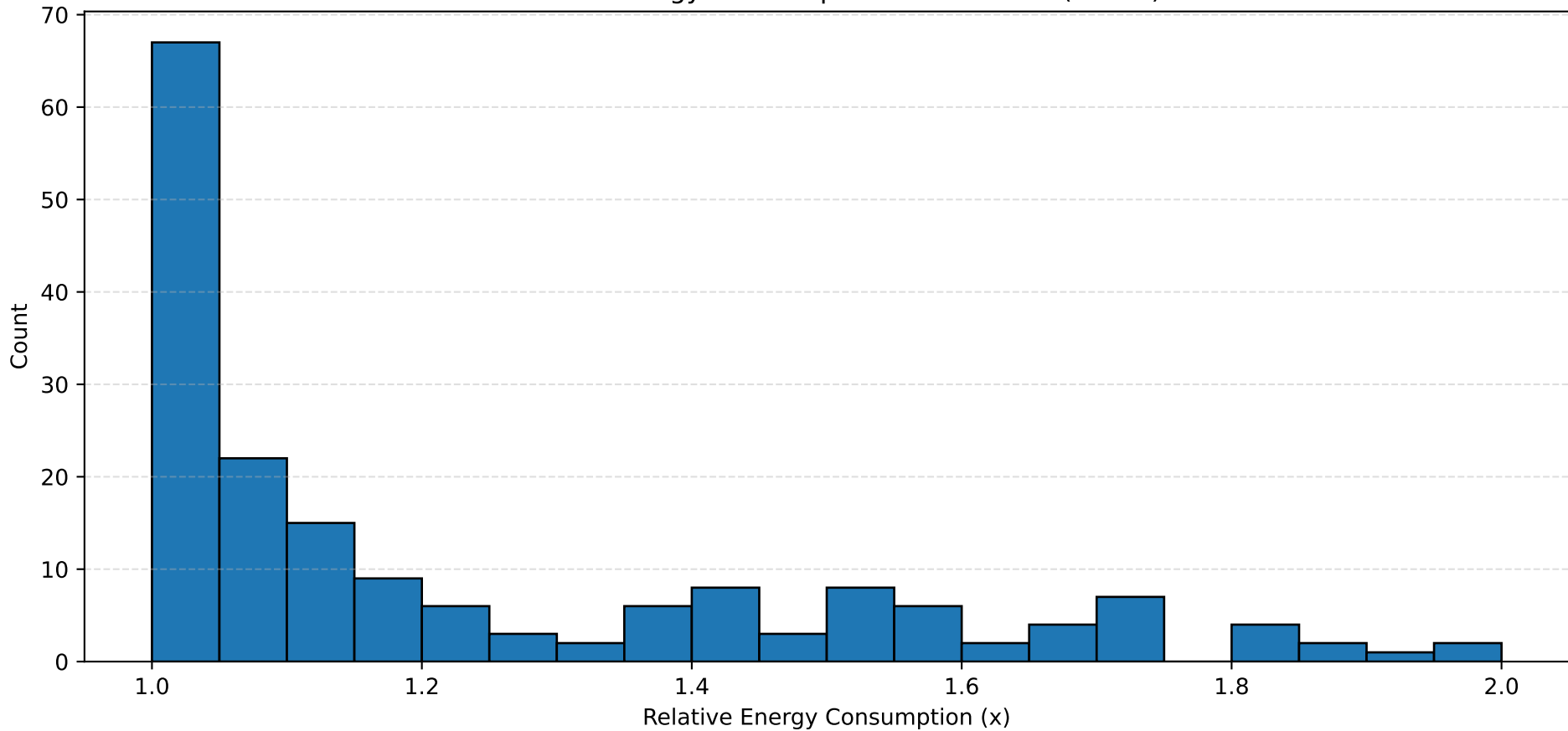
Relative Energy Consumption Distribution (1x-2x)
