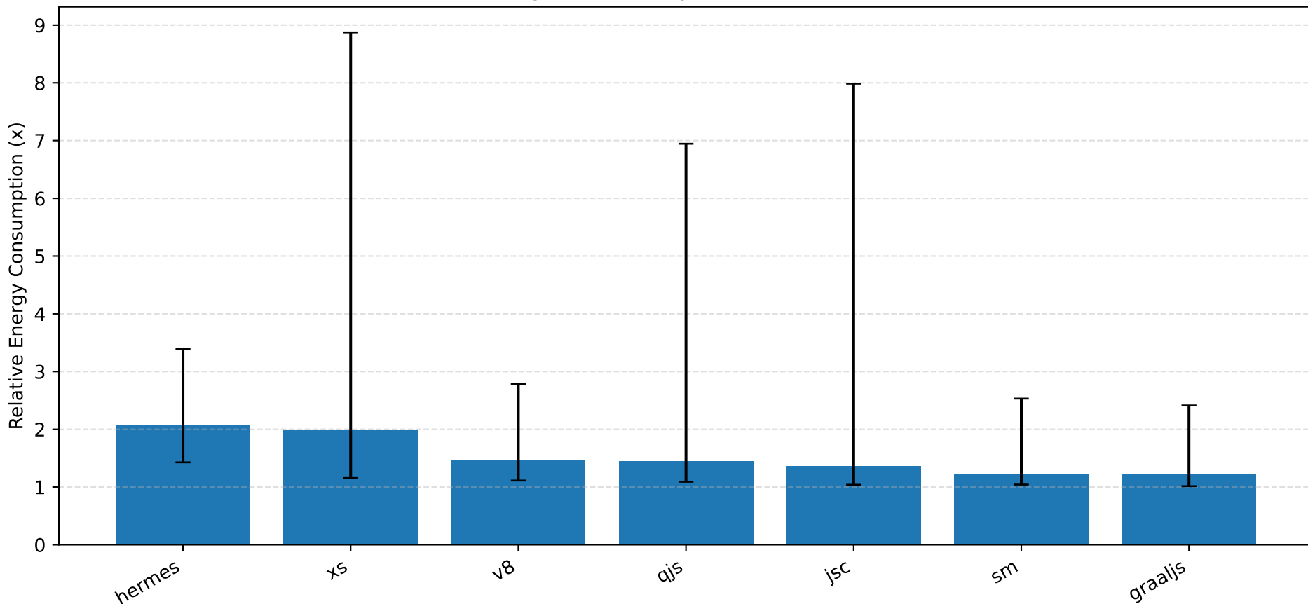
Engine Efficiency (Median + IQR)
