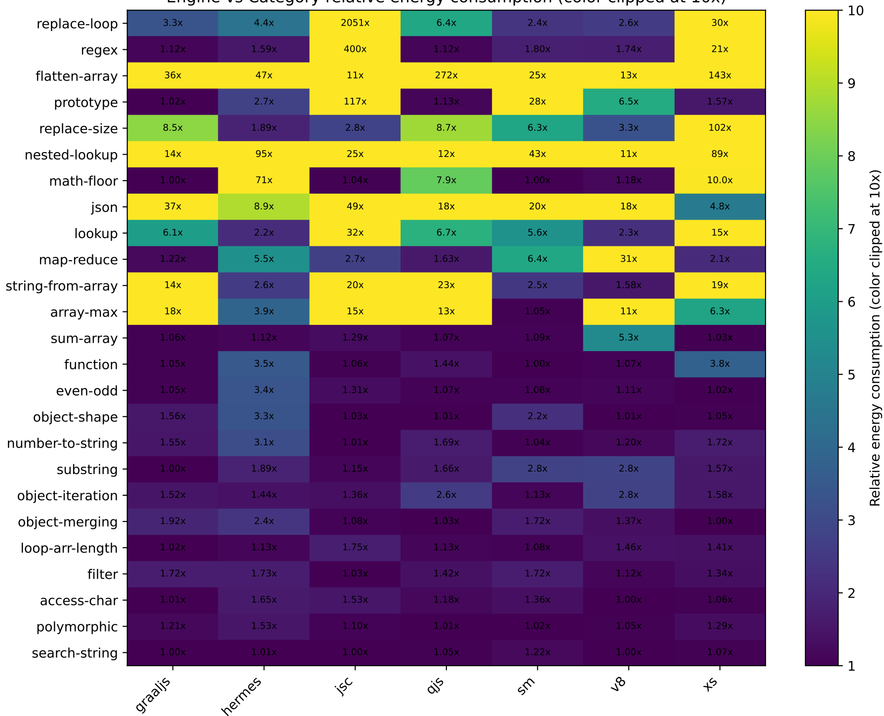
Engine vs Category relative energy consumption (color clipped at 10x)
