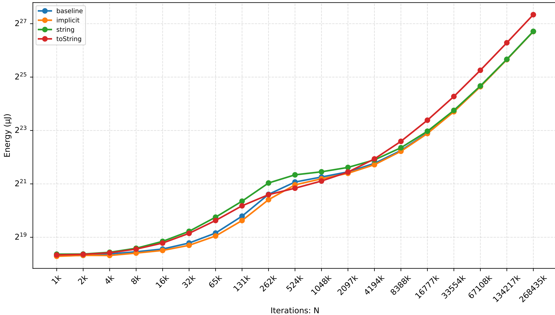
GRAALJS — number-to-string Scaling
