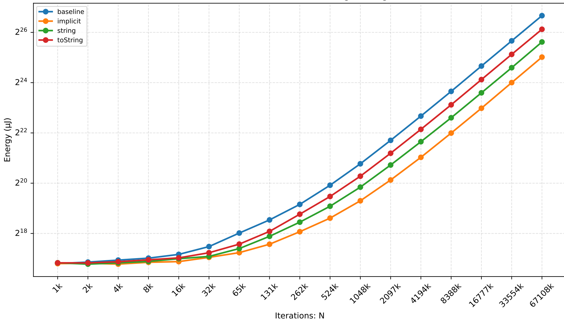
HERMES — number-to-string Scaling
