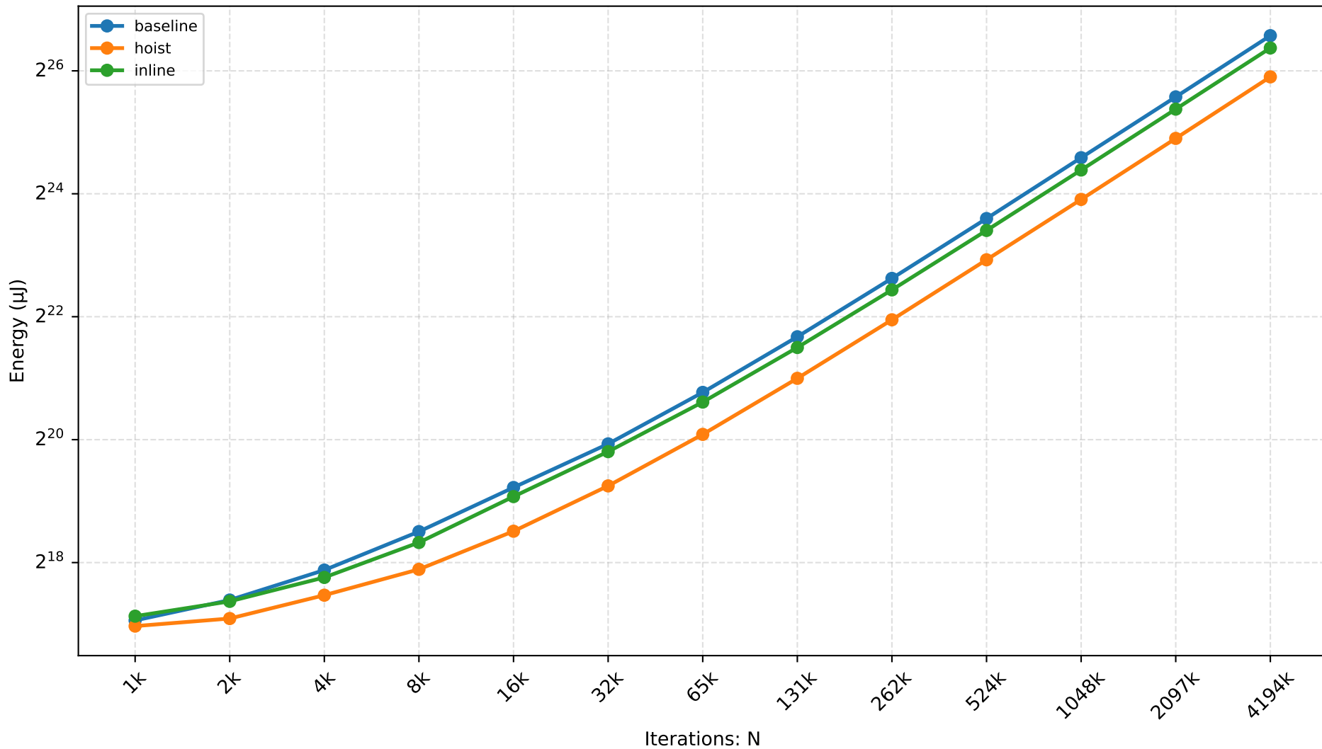
HERMES — regex Scaling
