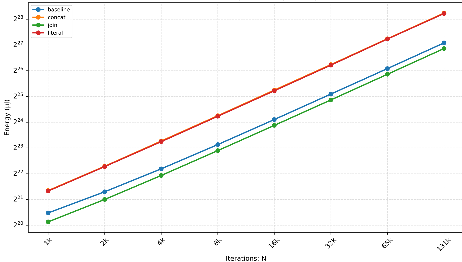
HERMES — string-from-array Scaling
