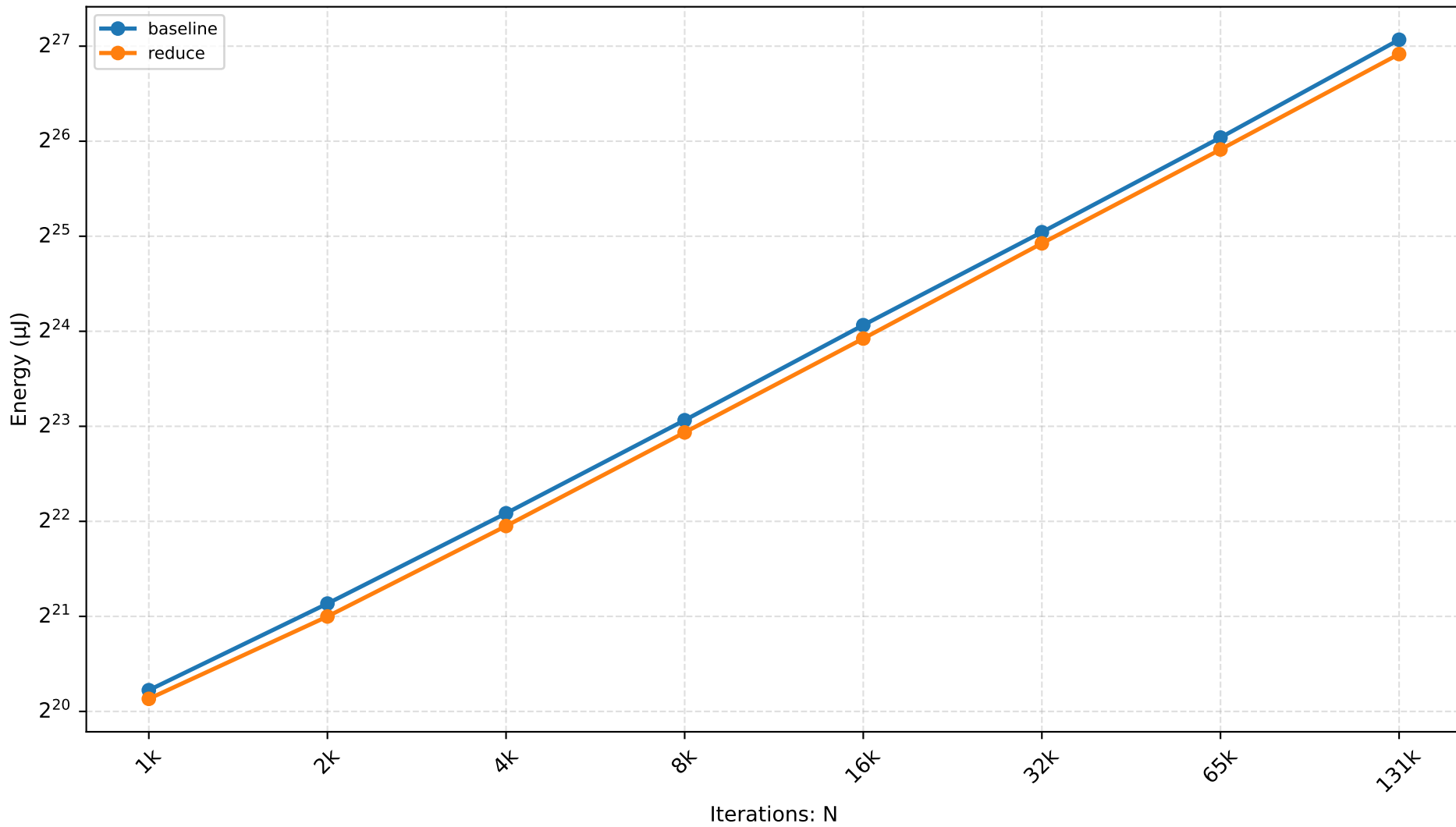
HERMES — sum-array Scaling
