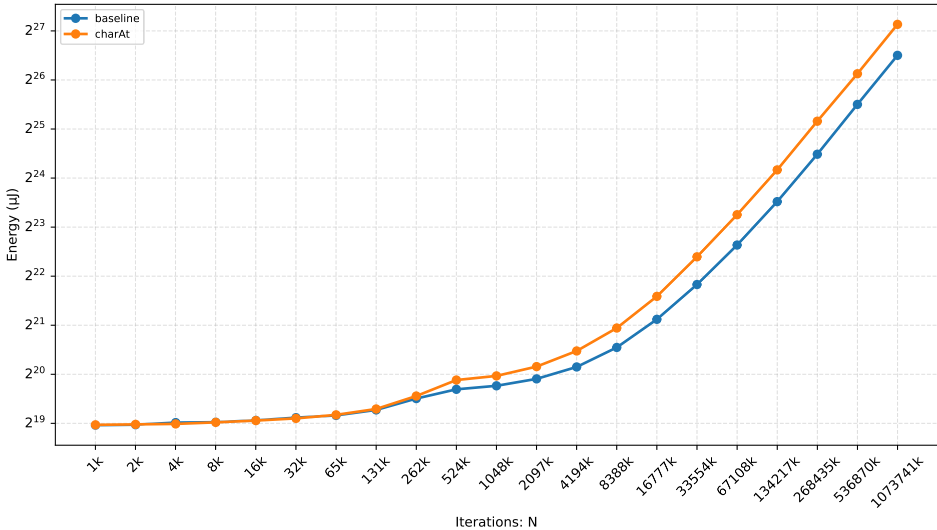
JSC — access-char Scaling
