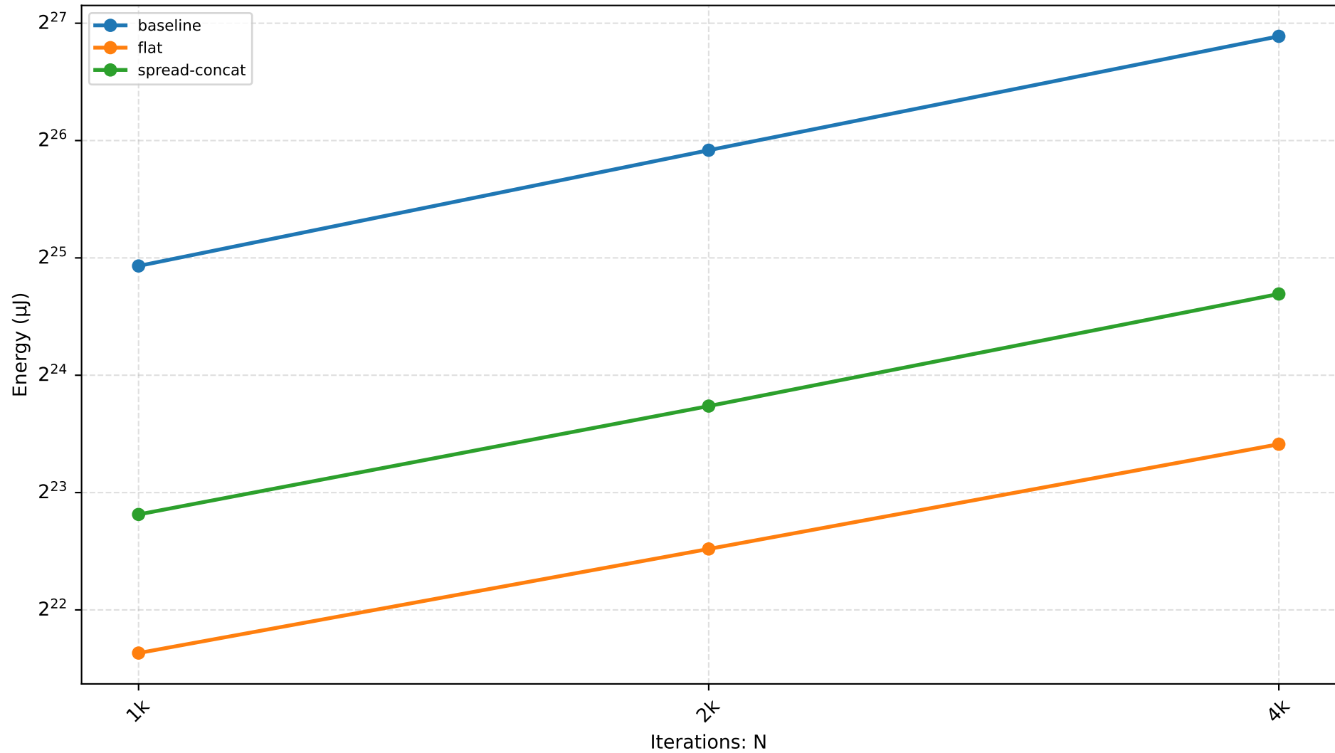
JSC — flatten-array Scaling
