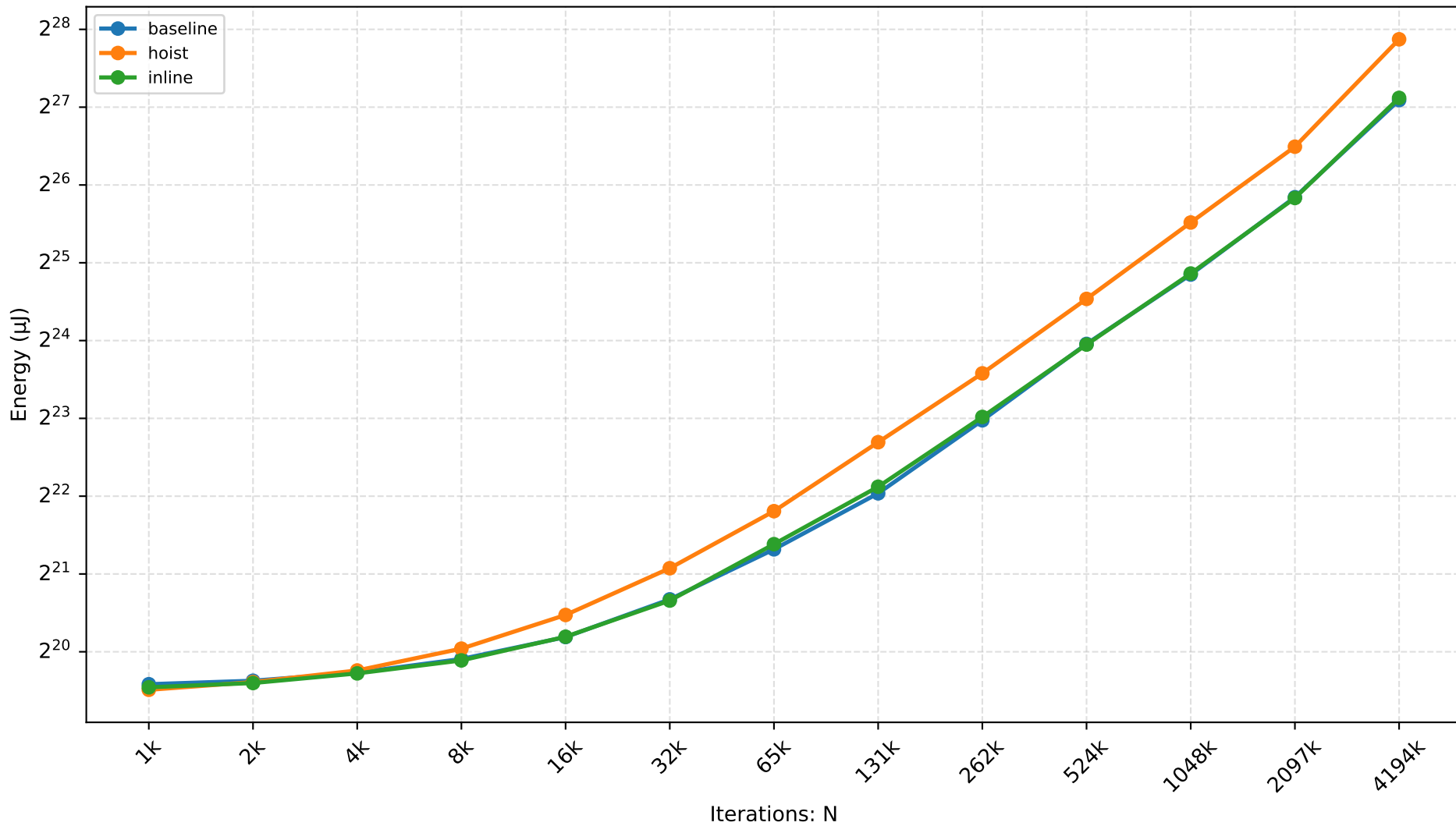
JSC — loop-arr-length Scaling
