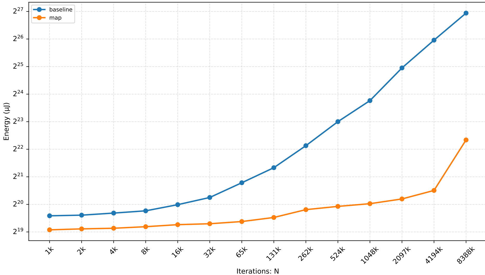
JSC — nested-lookup Scaling
