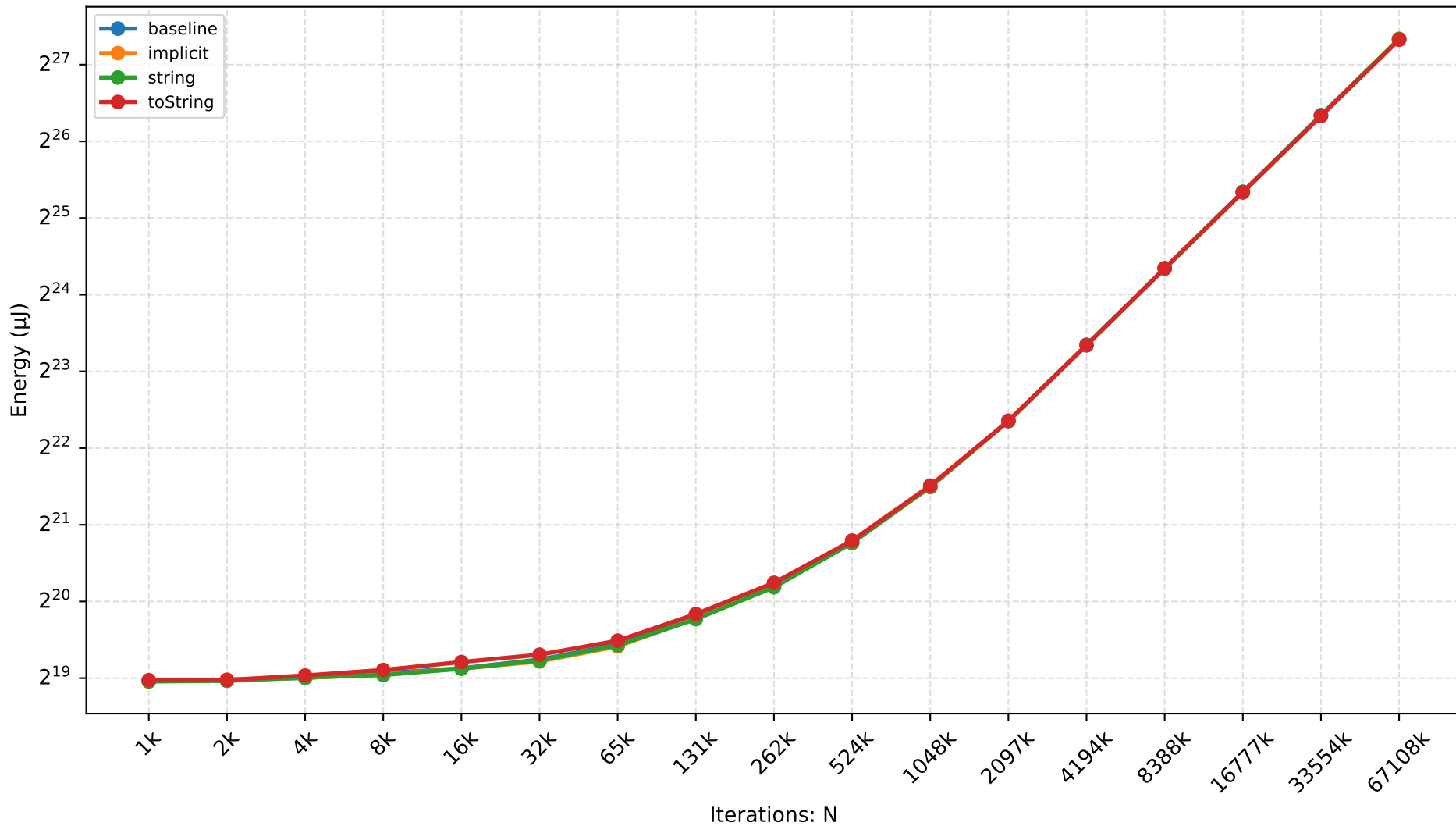
JSC — number-to-string Scaling
