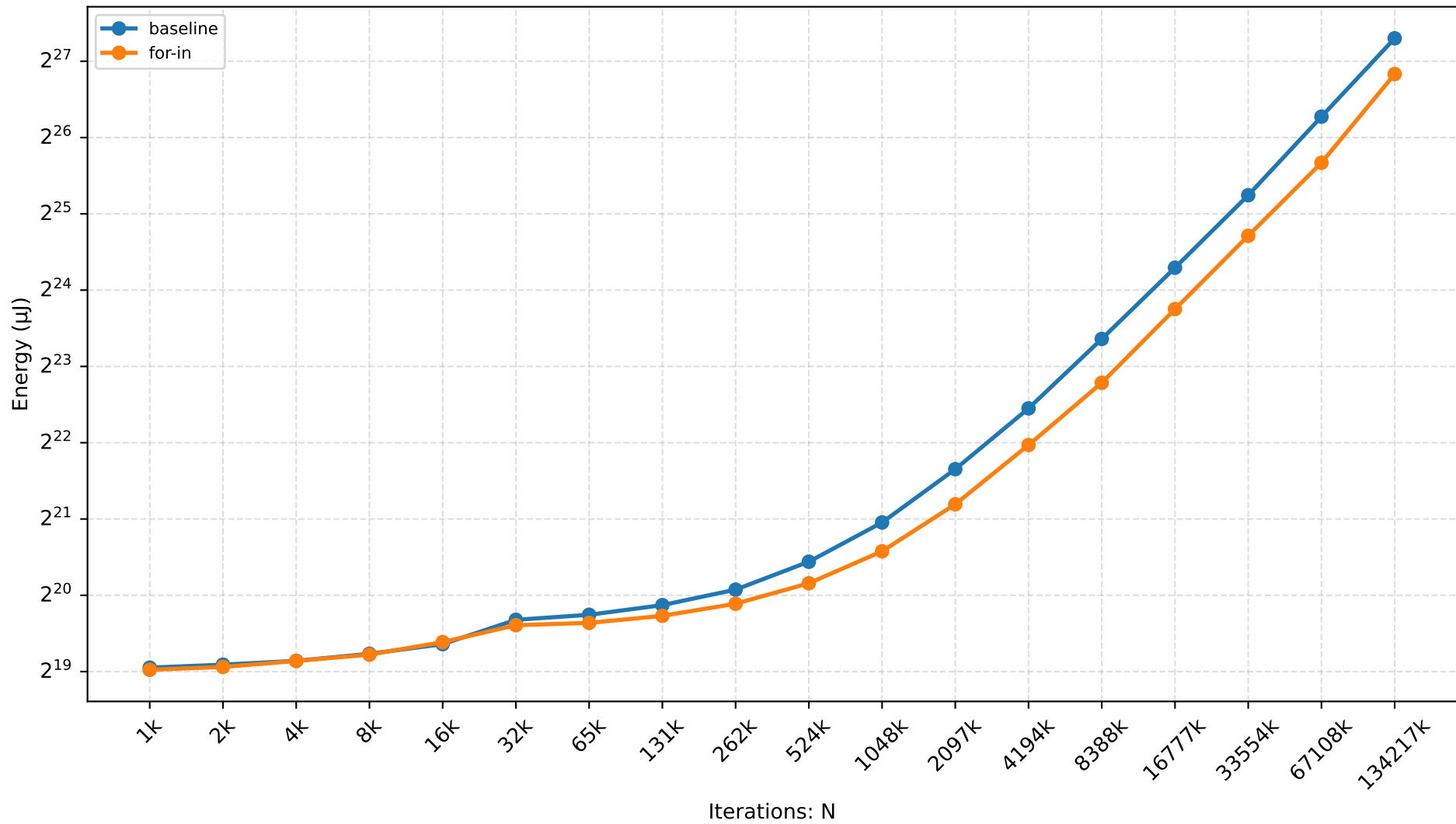
JSC — object-iteration Scaling
