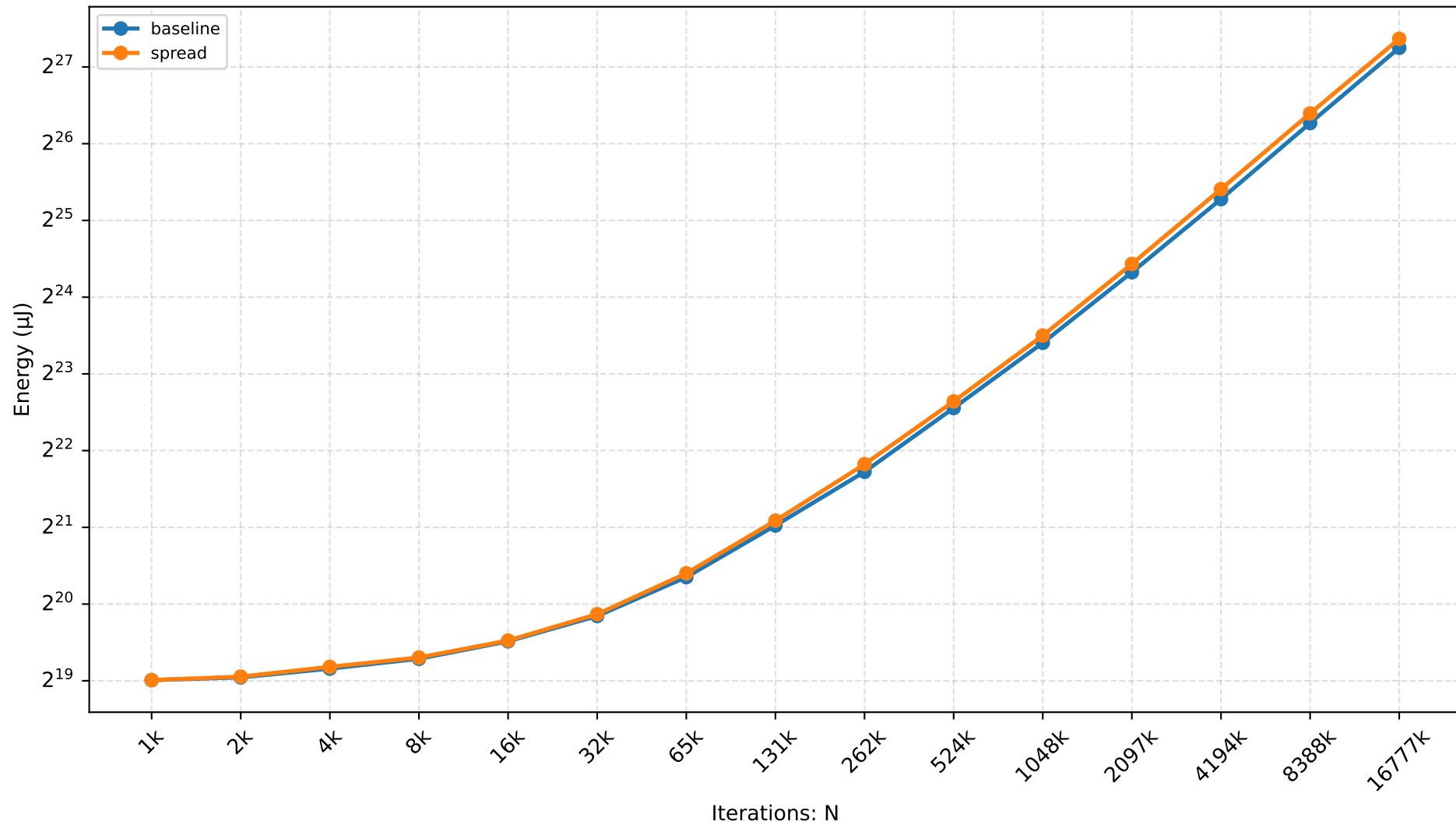
JSC — object-merging Scaling
