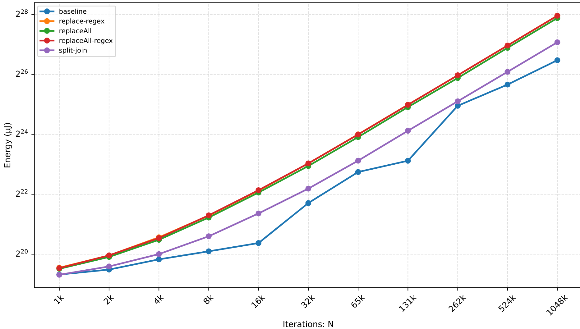
JSC — replace-size Scaling
