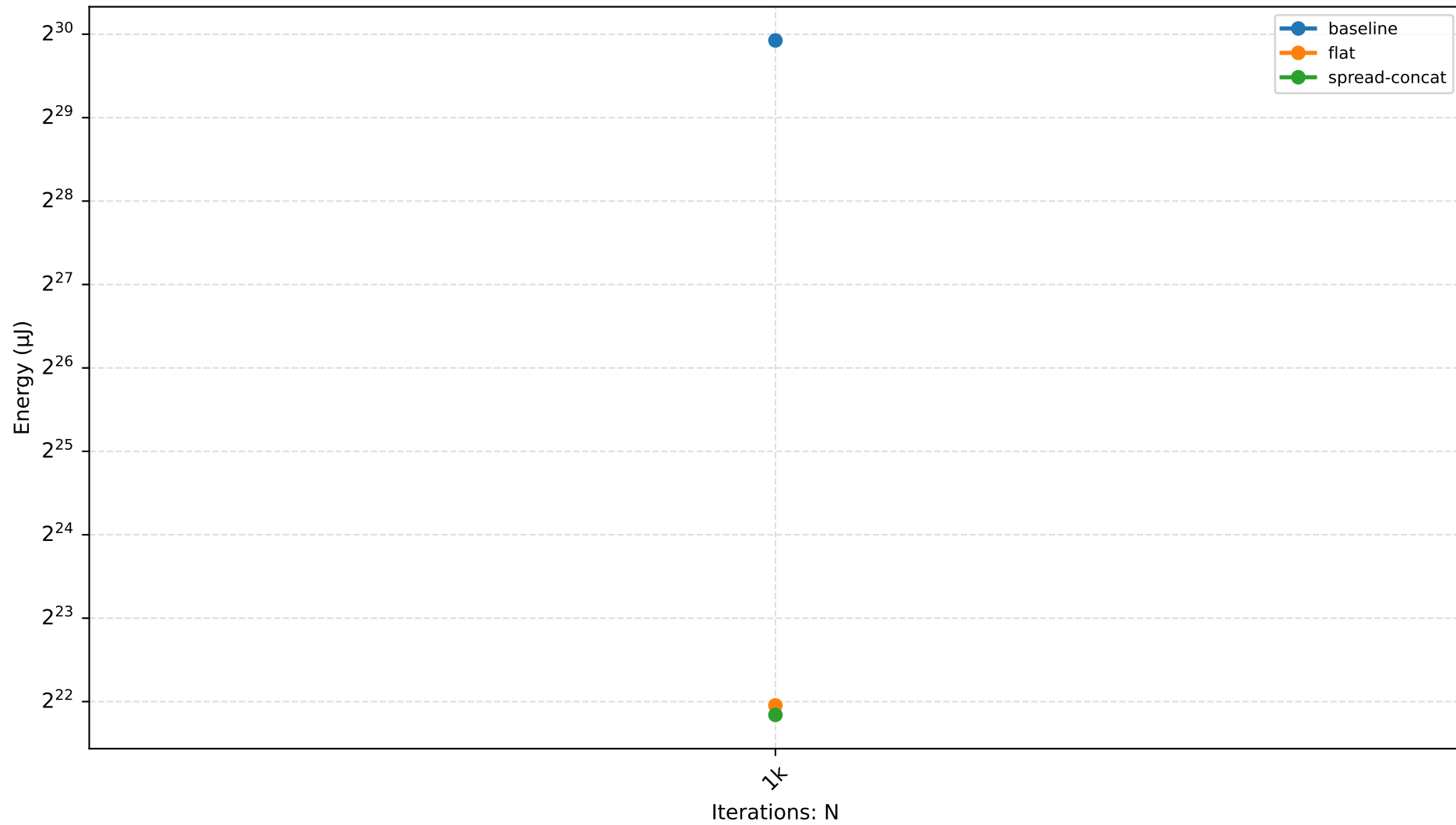
QJS — flatten-array Scaling
