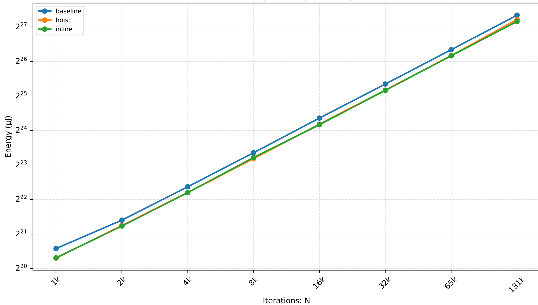
QJS — loop-arr-length Scaling
