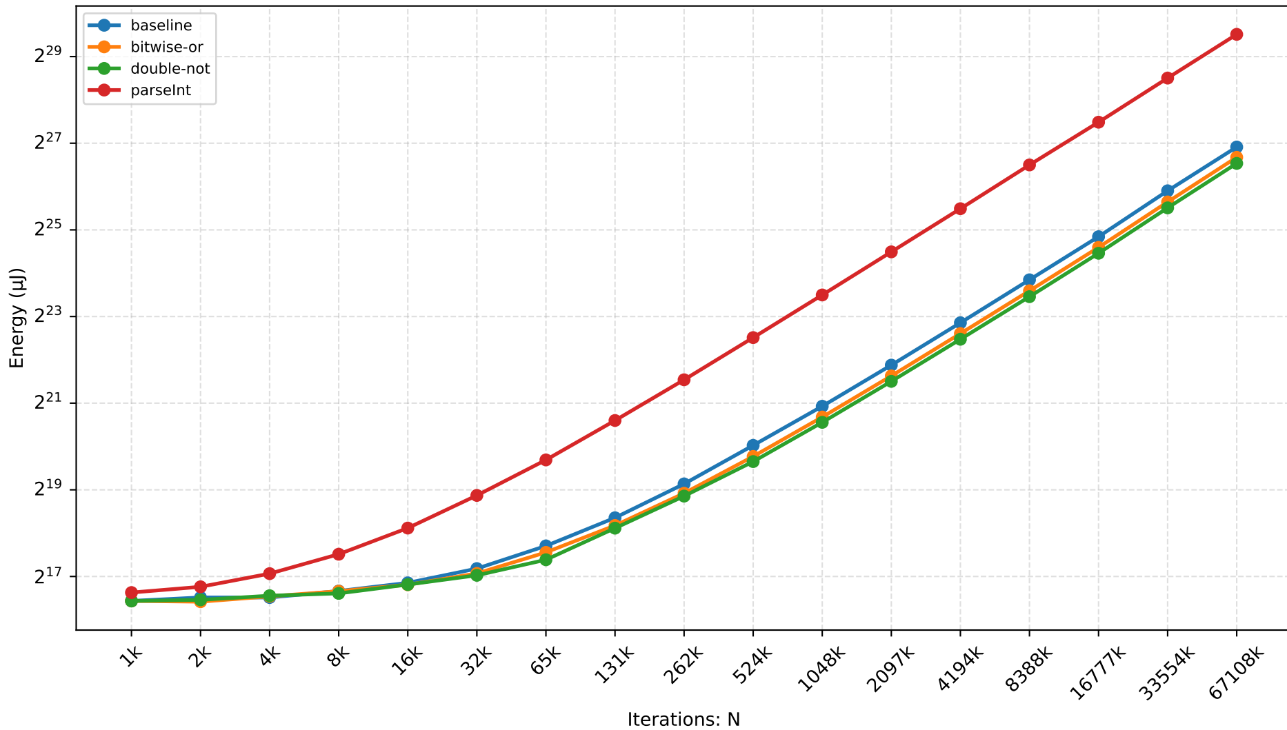
QJS — math-floor Scaling
