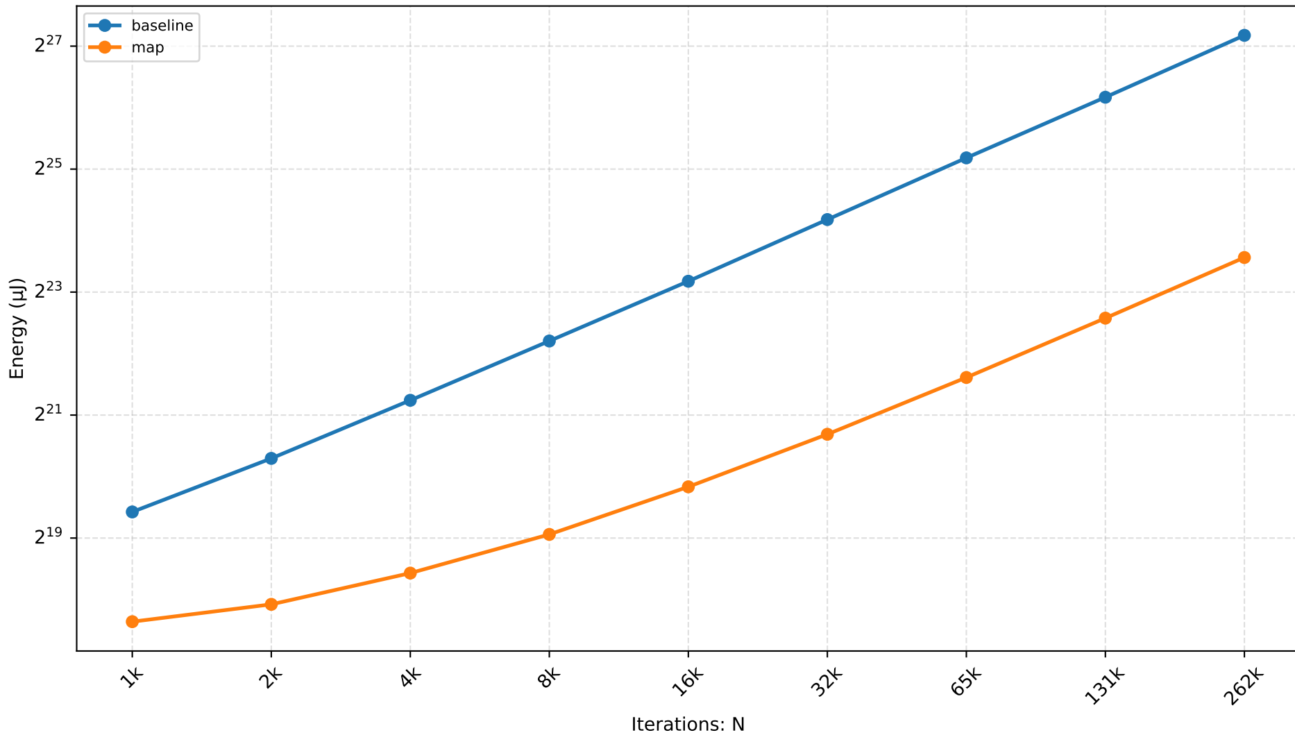
QJS — nested-lookup Scaling
