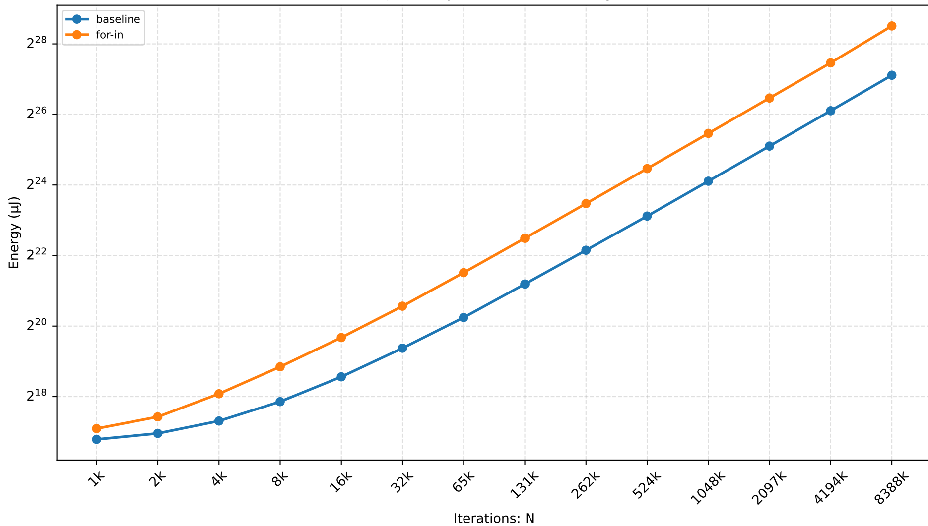
QJS — object-iteration Scaling
