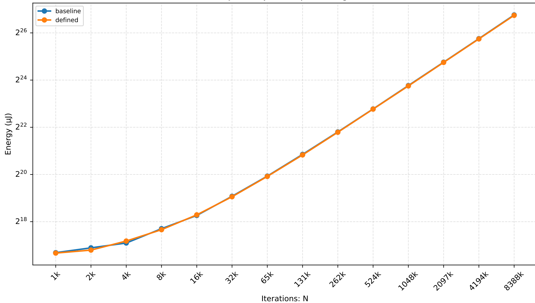
QJS — object-shape Scaling
