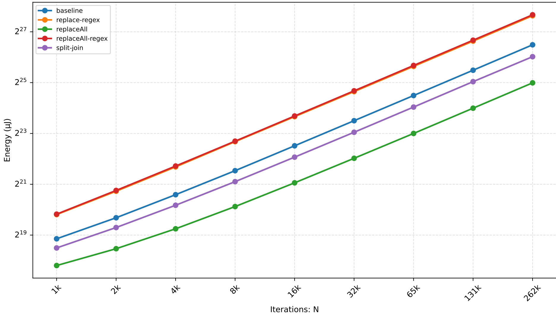
QJS — replace-loop Scaling
