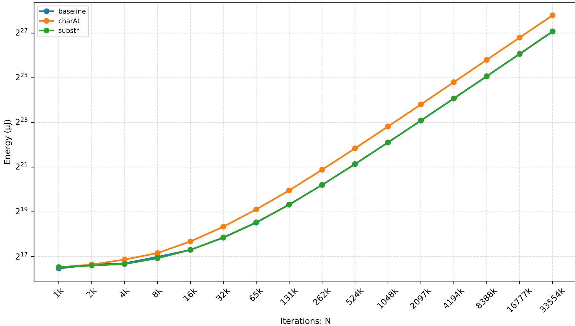
QJS — substring Scaling
