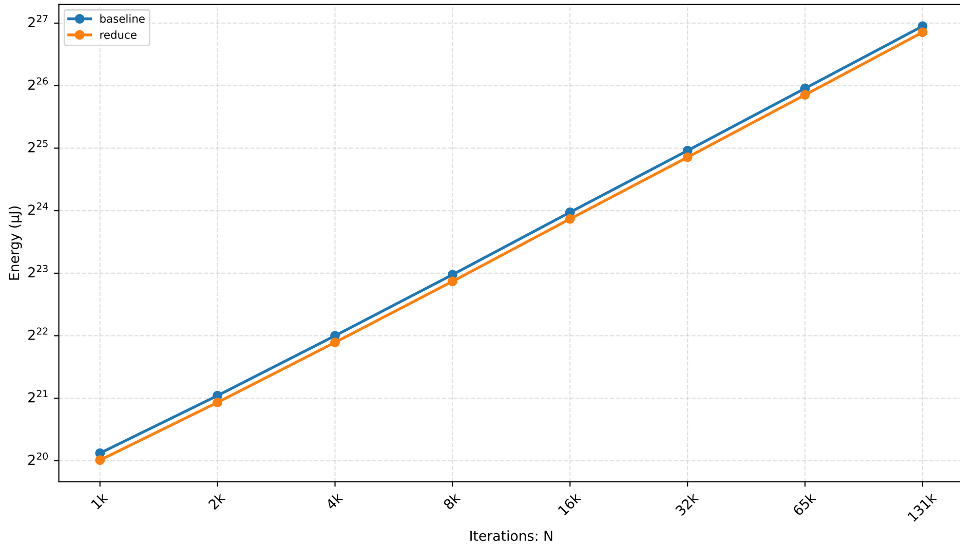
QJS — sum-array Scaling
