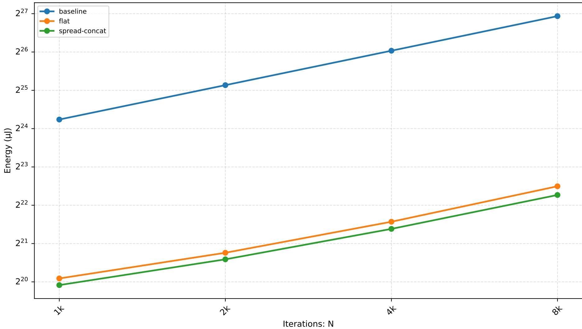
SM — flatten-array Scaling
