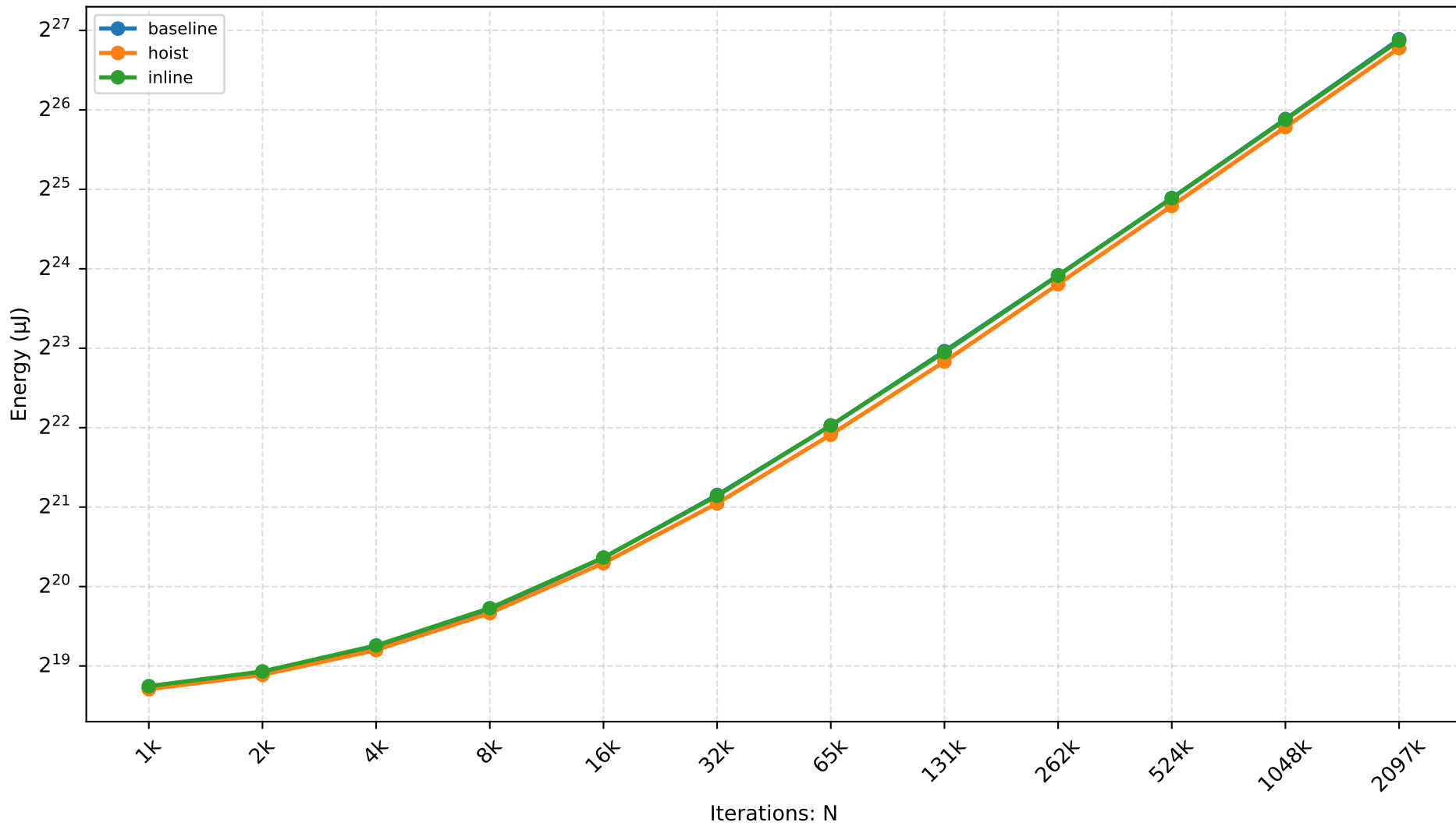
SM — loop-arr-length Scaling
