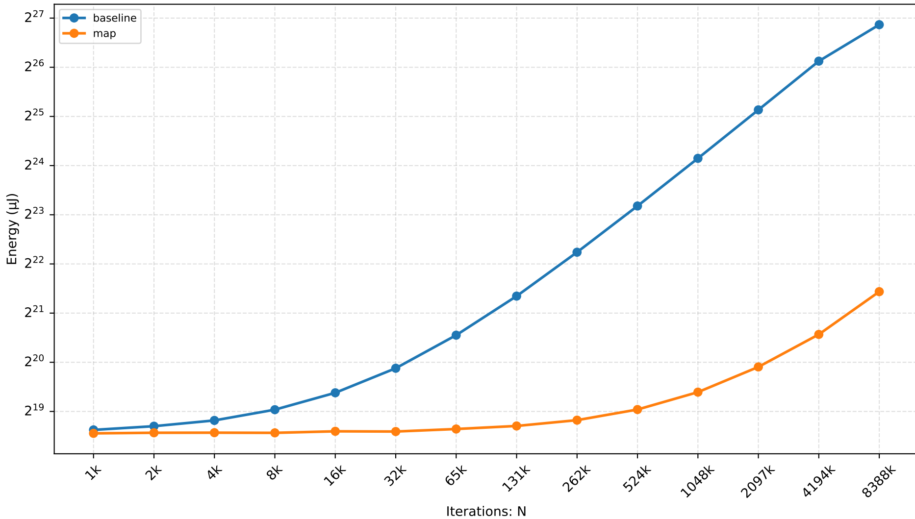
SM — nested-lookup Scaling
