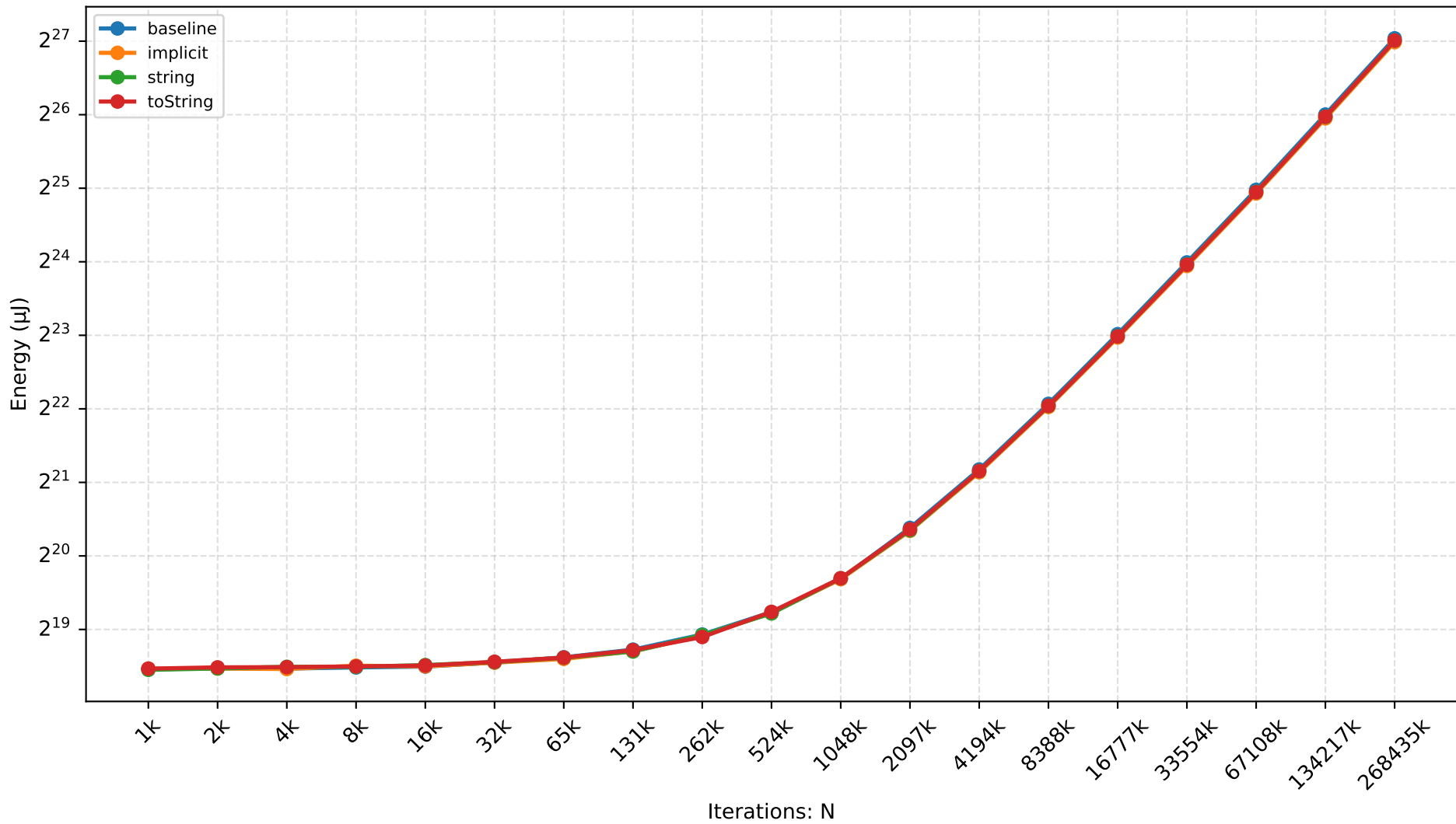
SM — number-to-string Scaling
