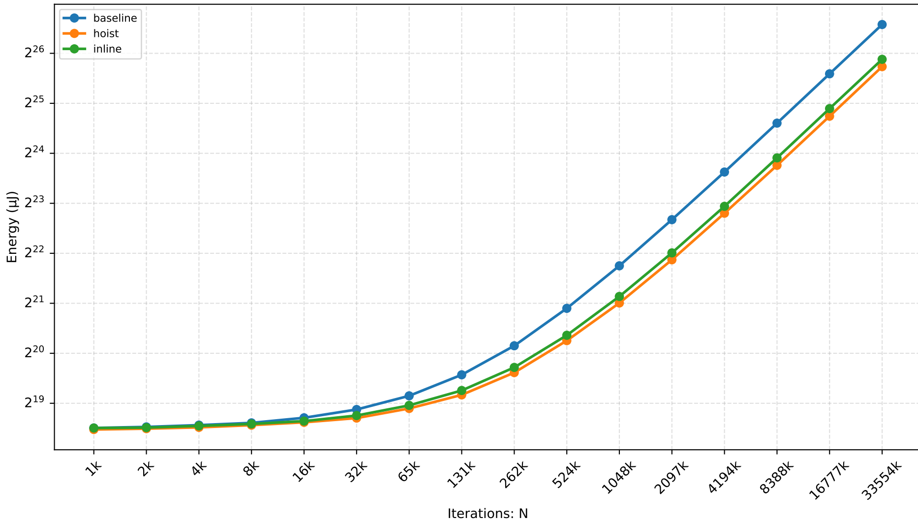
SM — regex Scaling
