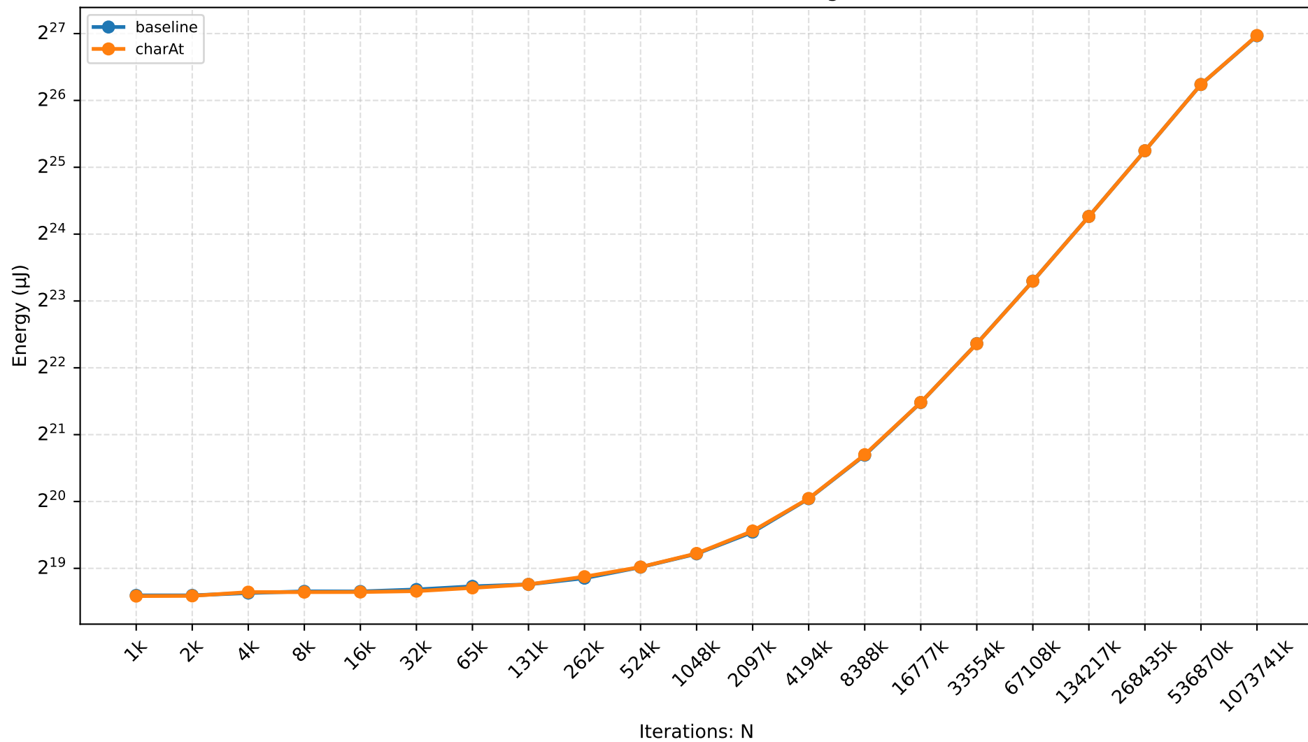
V8 — access-char Scaling
