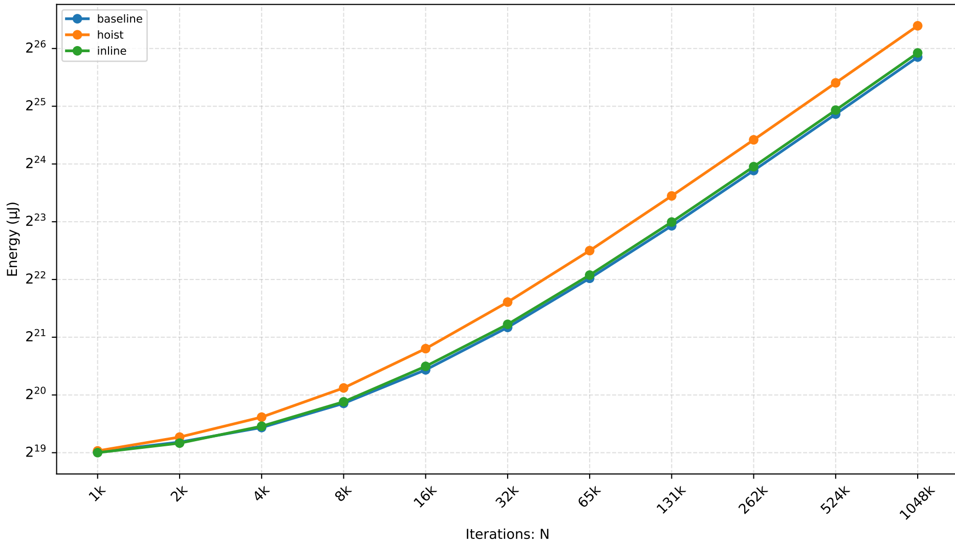
V8 — loop-arr-length Scaling
