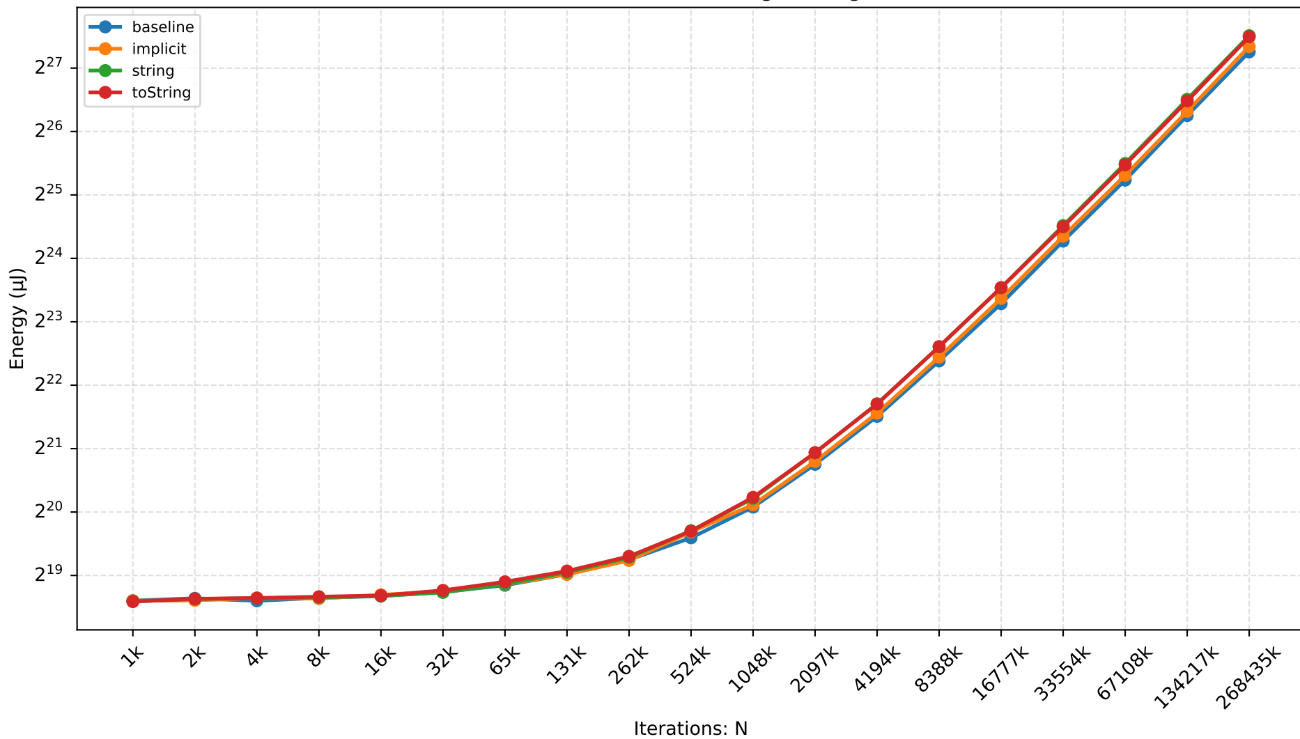
V8 — number-to-string Scaling
