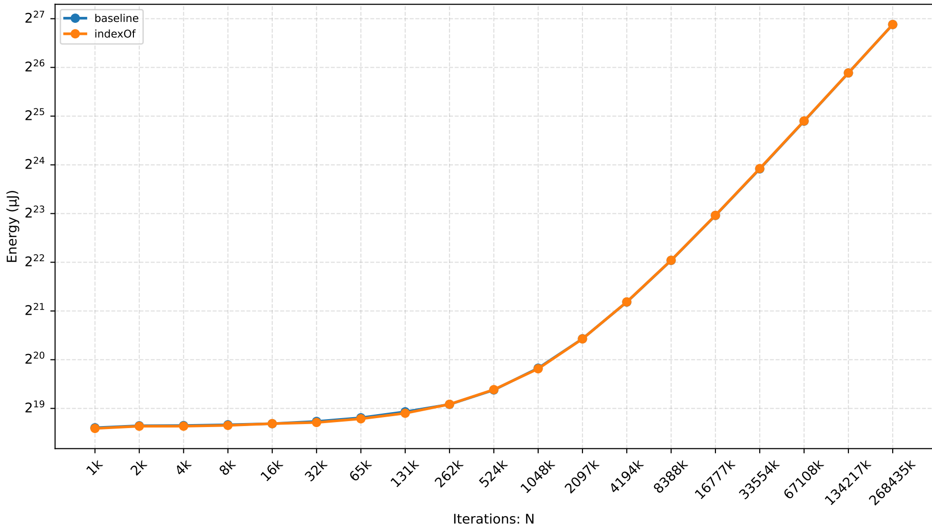
V8 — search-string Scaling
