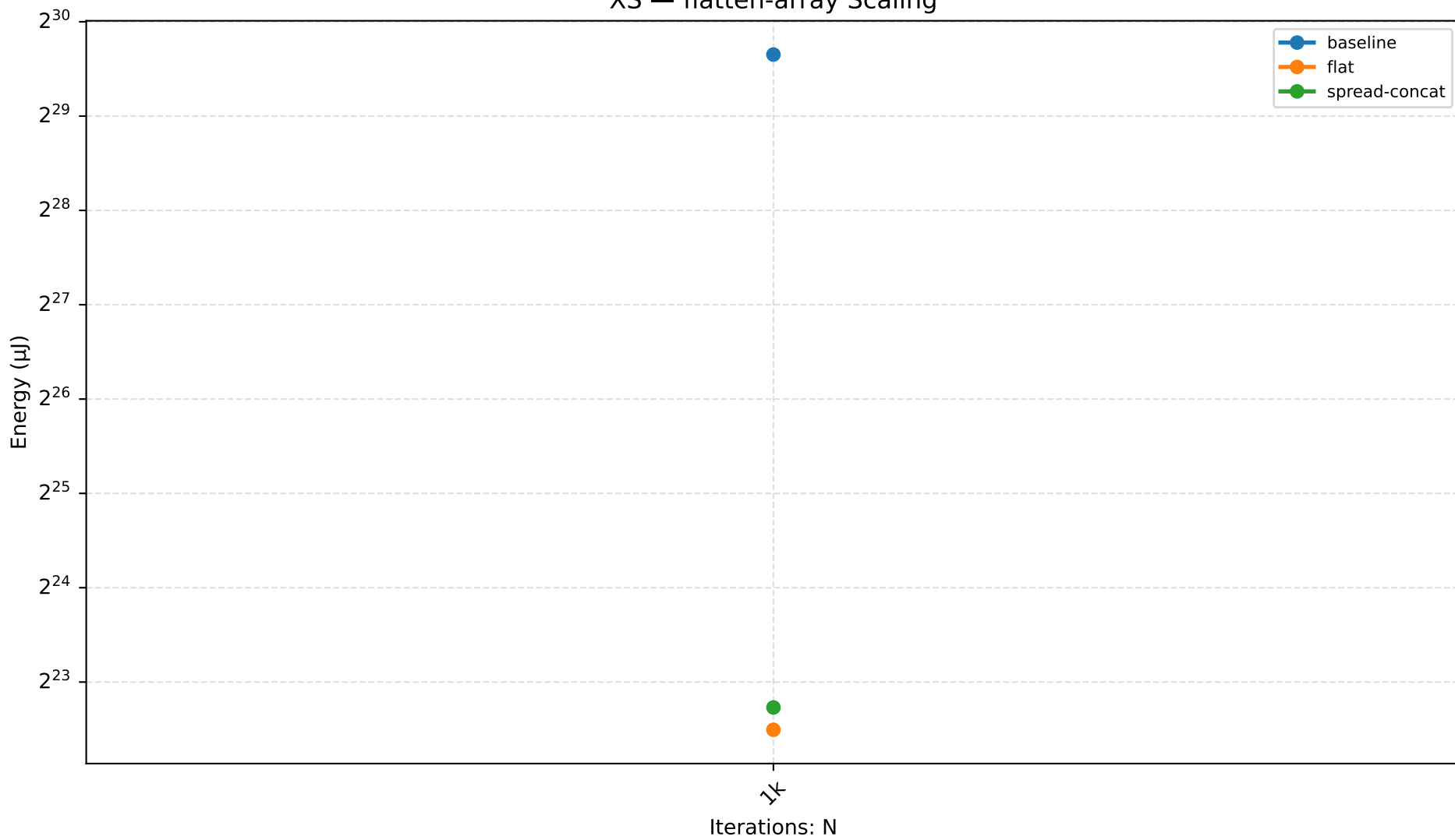
XS — flatten-array Scaling
