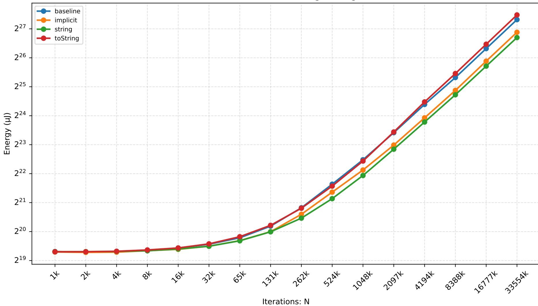
XS — number-to-string Scaling
